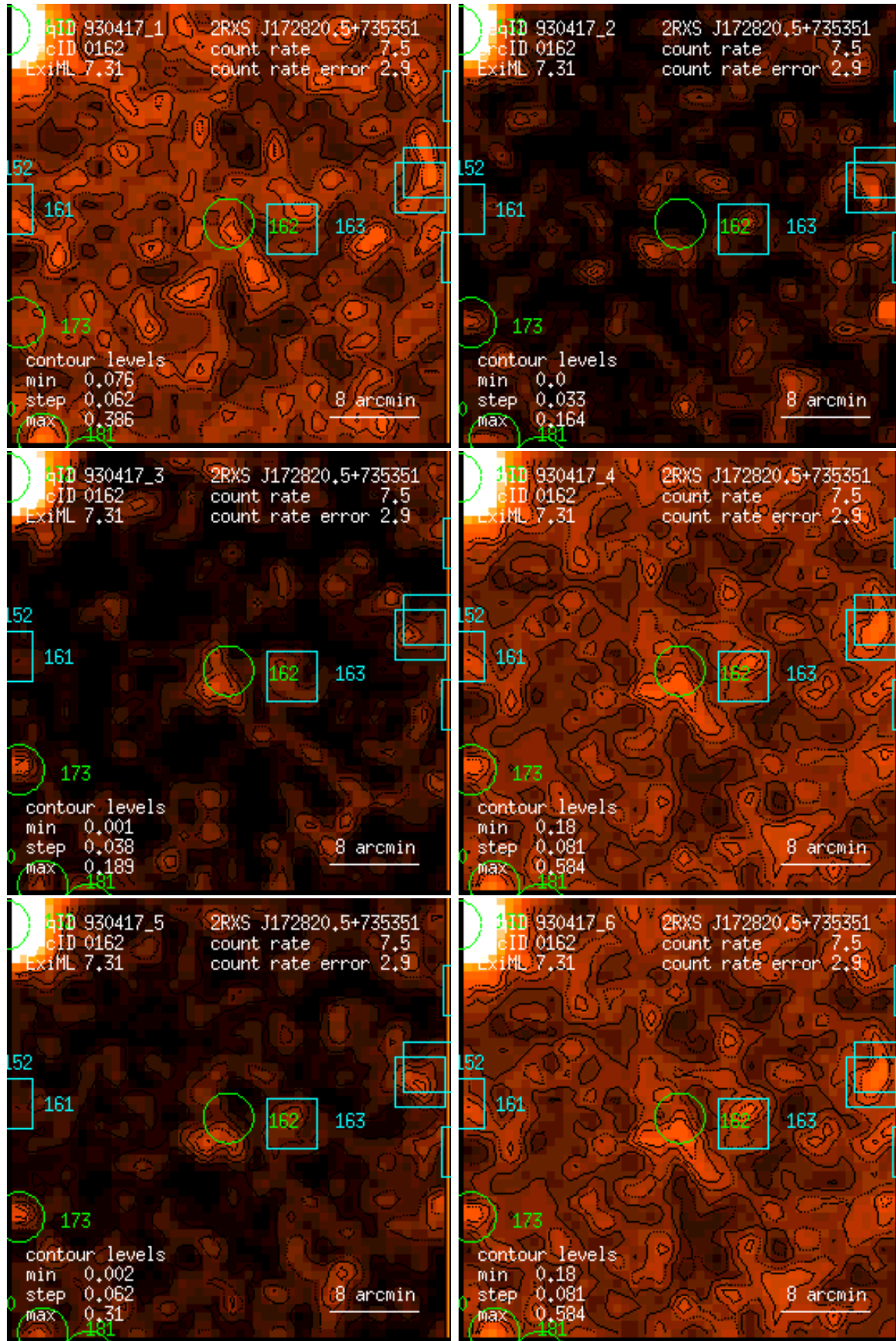
Figure 162: RASS 930417: detection 0162: band rate images, Gaussian filter: (1) PSPC channels 11 – 41, (2) 52 – 90, (3) 91 – 201, (4) 11 – 235, (5) 52 – 201, (6) 11 – 201. Broad band rates in counts/ks. Band rate contour levels in counts/ks/arcmin 2 .
