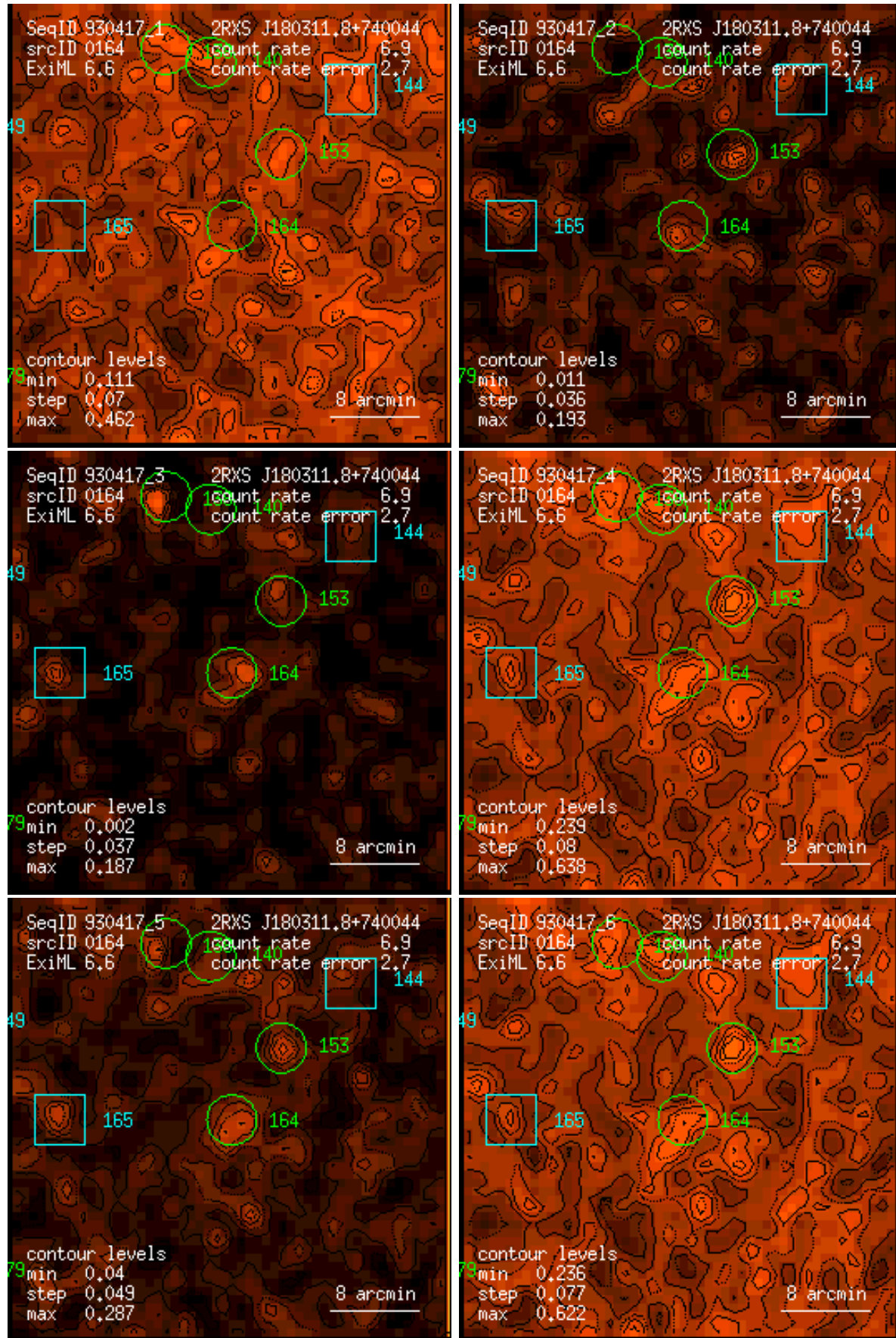
Figure 164: RASS 930417: detection 0164: band rate images, Gaussian filter: (1) PSPC channels 11 – 41, (2) 52 – 90, (3) 91 – 201, (4) 11 – 235, (5) 52 – 201, (6) 11 – 201. Broad band rates in counts/ks. Band rate contour levels in counts/ks/arcmin 2 .
