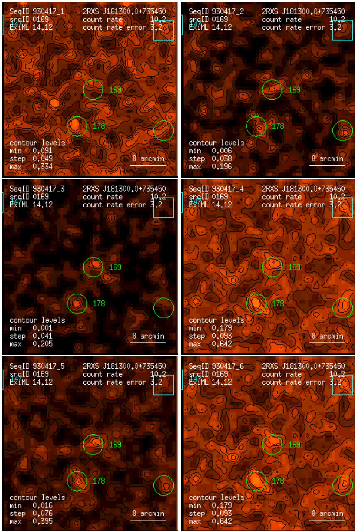
Figure 169: RASS 930417: detection 0169: band rate images, Gaussian filter: (1) PSPC channels 11 – 41, (2) 52 – 90, (3) 91 – 201, (4) 11 – 235, (5) 52 – 201, (6) 11 – 201. Broad band rates in counts/ks. Band rate contour levels in counts/ks/arcmin 2 .
