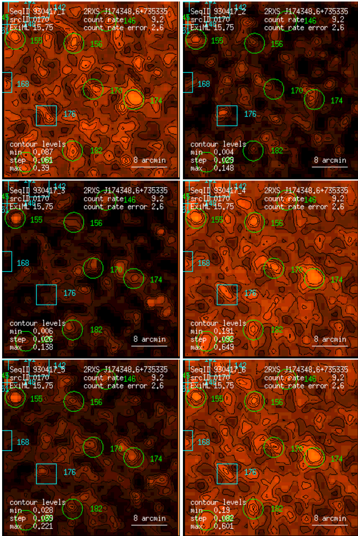
Figure 170: RASS 930417: detection 0170: band rate images, Gaussian filter: (1) PSPC channels 11 – 41, (2) 52 – 90, (3) 91 – 201, (4) 11 – 235, (5) 52 – 201, (6) 11 – 201. Broad band rates in counts/ks. Band rate contour levels in counts/ks/arcmin 2 .
