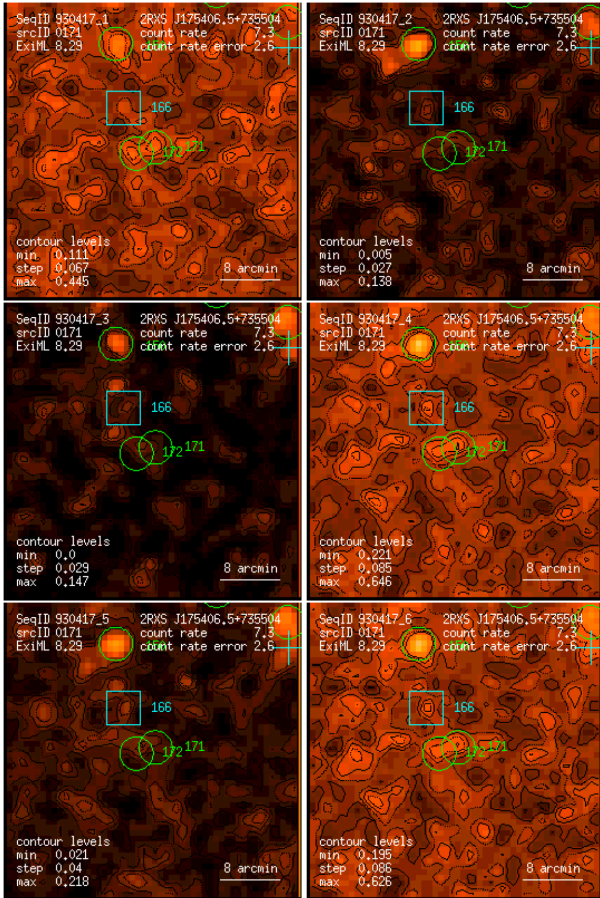
Figure 171: RASS 930417: detection 0171: band rate images, Gaussian filter: (1) PSPC channels 11 – 41, (2) 52 – 90, (3) 91 – 201, (4) 11 – 235, (5) 52 – 201, (6) 11 – 201. Broad band rates in counts/ks. Band rate contour levels in counts/ks/arcmin 2 .
