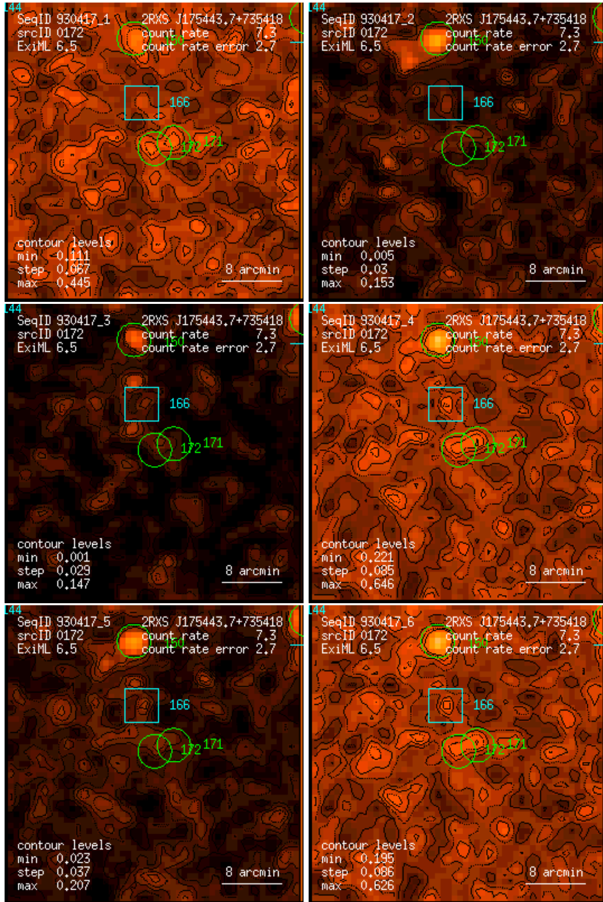
Figure 172: RASS 930417: detection 0172: band rate images, Gaussian filter: (1) PSPC channels 11 – 41, (2) 52 – 90, (3) 91 – 201, (4) 11 – 235, (5) 52 – 201, (6) 11 – 201. Broad band rates in counts/ks. Band rate contour levels in counts/ks/arcmin 2 .
