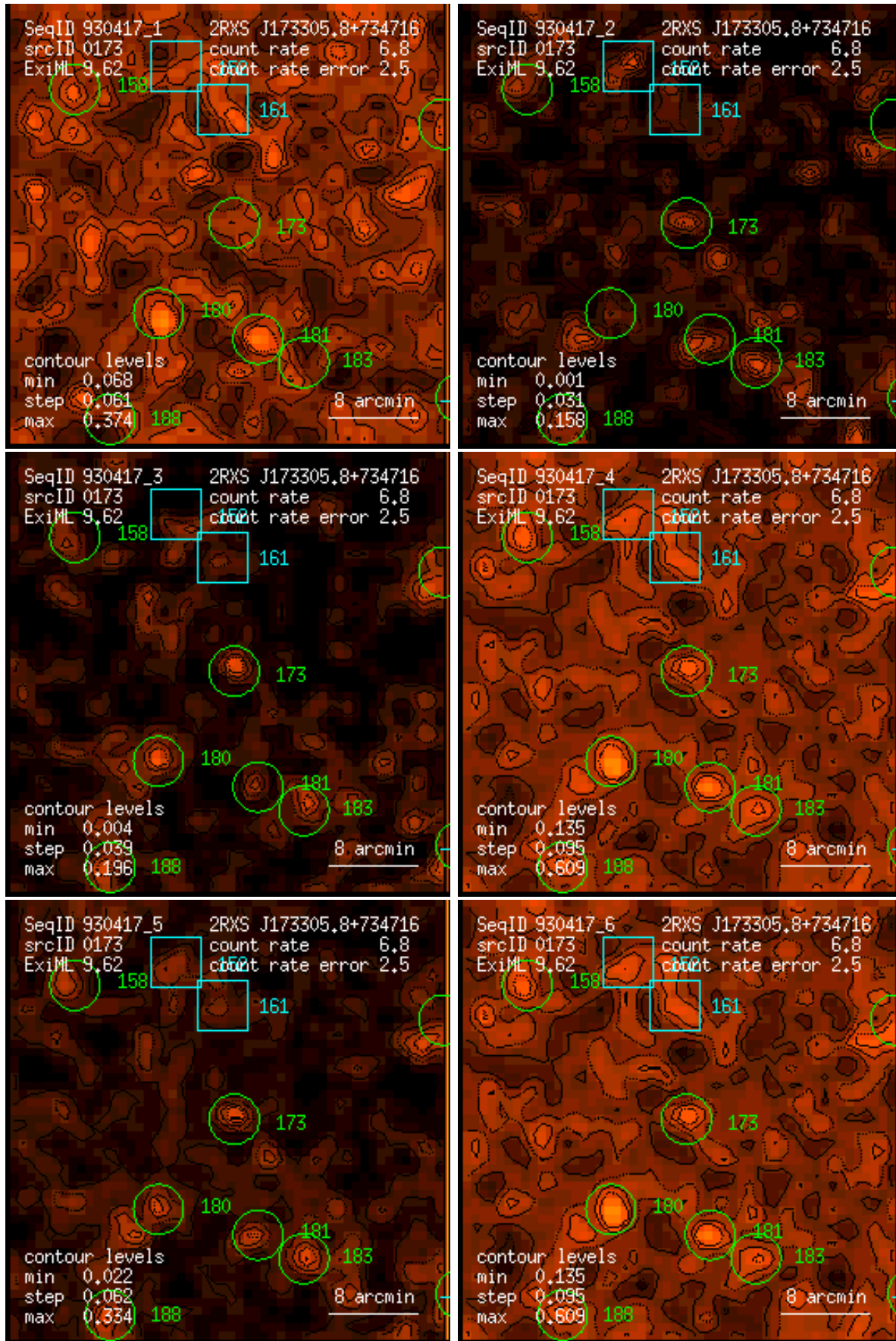
Figure 173: RASS 930417: detection 0173: band rate images, Gaussian filter: (1) PSPC channels 11 – 41, (2) 52 – 90, (3) 91 – 201, (4) 11 – 235, (5) 52 – 201, (6) 11 – 201. Broad band rates in counts/ks. Band rate contour levels in counts/ks/arcmin 2 .
