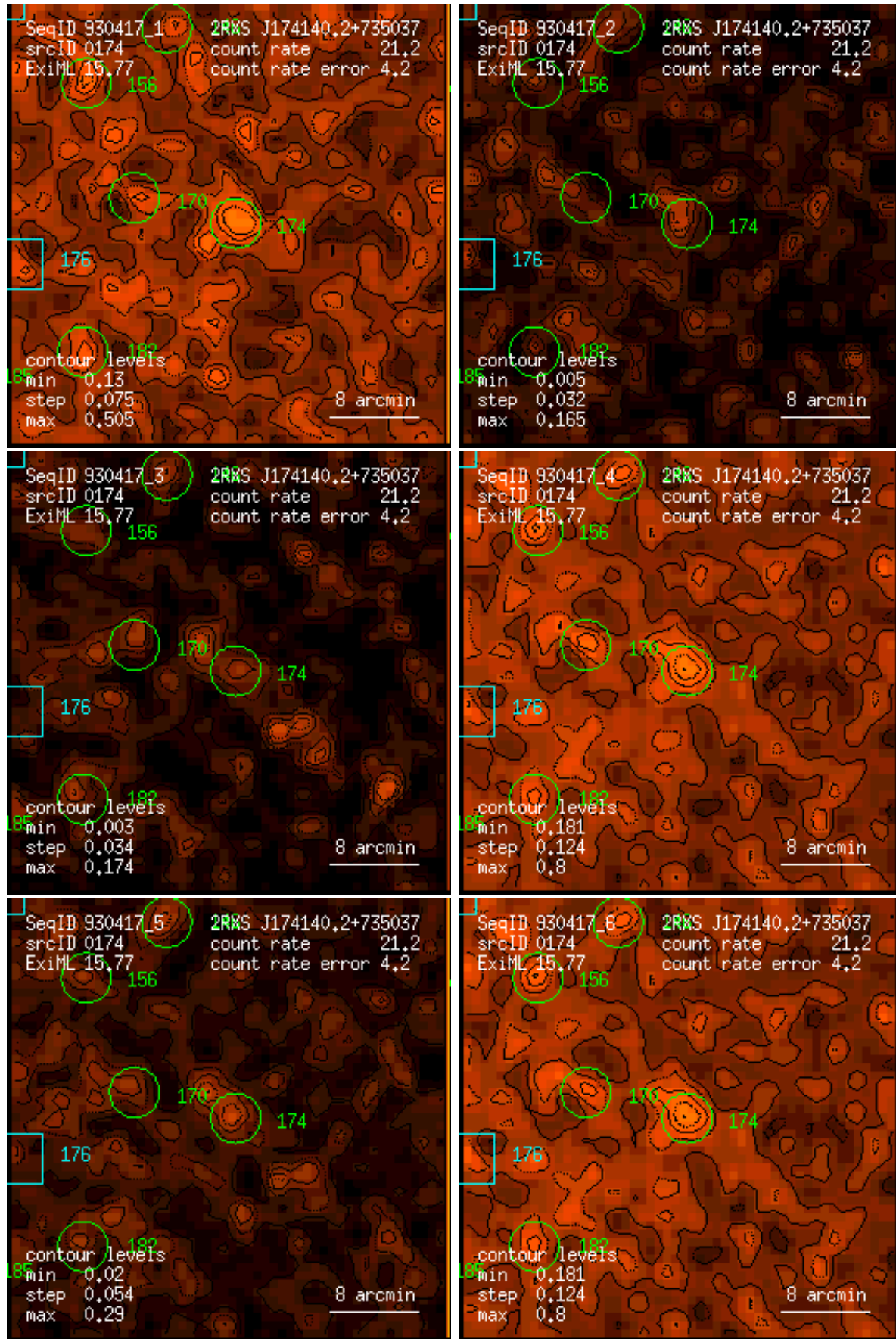
Figure 174: RASS 930417: detection 0174: band rate images, Gaussian filter: (1) PSPC channels 11 – 41, (2) 52 – 90, (3) 91 – 201, (4) 11 – 235, (5) 52 – 201, (6) 11 – 201. Broad band rates in counts/ks. Band rate contour levels in counts/ks/arcmin 2 .
