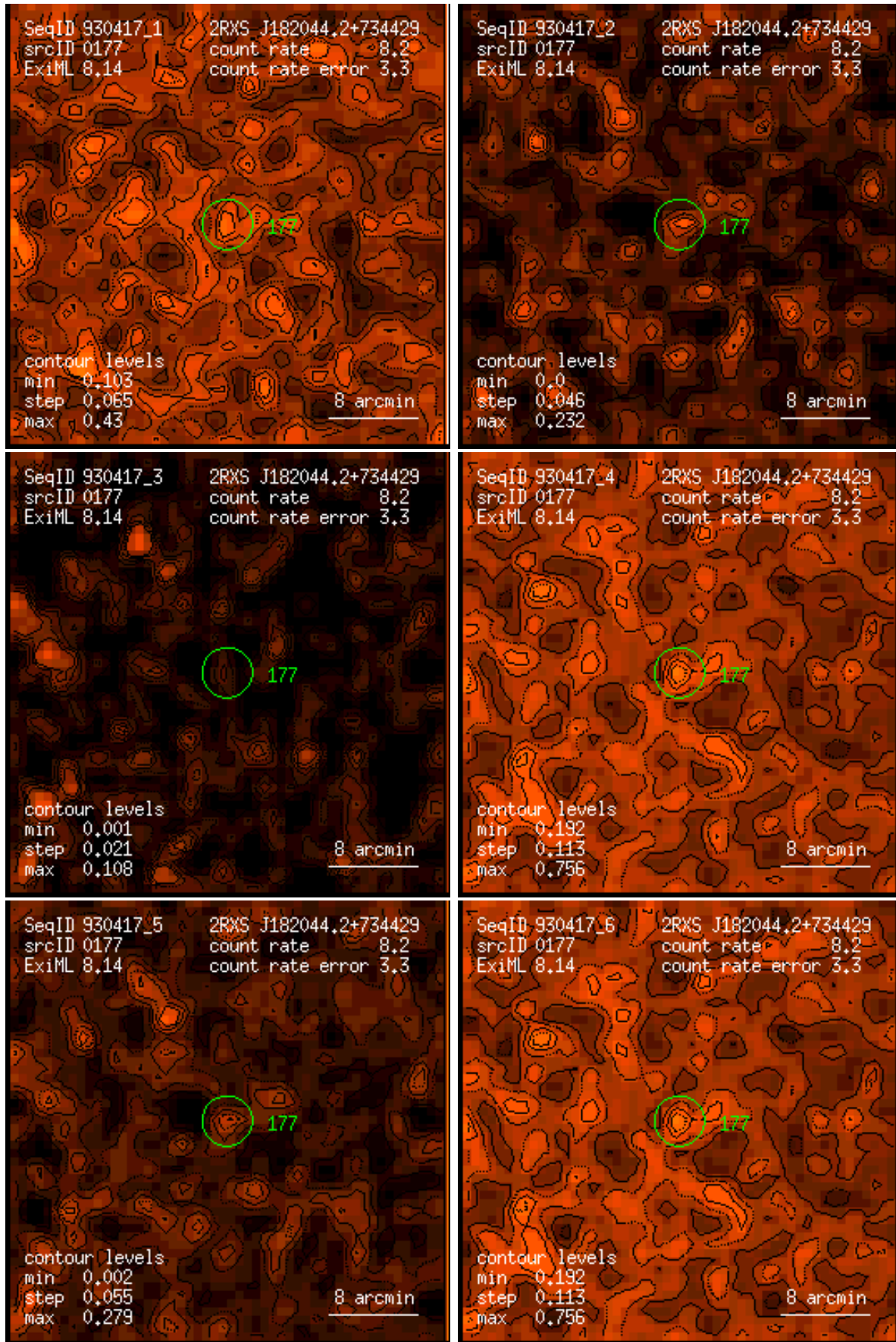
Figure 177: RASS 930417: detection 0177: band rate images, Gaussian filter: (1) PSPC channels 11 – 41, (2) 52 – 90, (3) 91 – 201, (4) 11 – 235, (5) 52 – 201, (6) 11 – 201. Broad band rates in counts/ks. Band rate contour levels in counts/ks/arcmin 2 .
