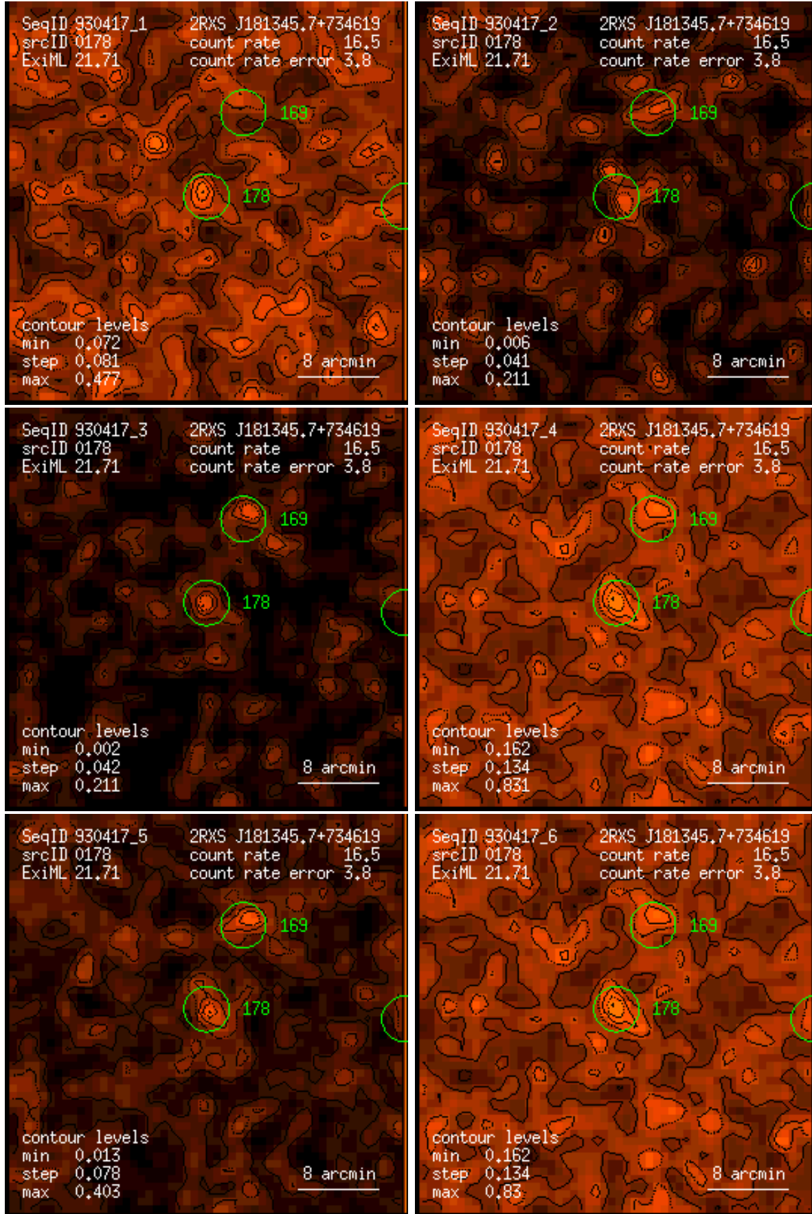
Figure 178: RASS 930417: detection 0178: band rate images, Gaussian filter: (1) PSPC channels 11 – 41, (2) 52 – 90, (3) 91 – 201, (4) 11 – 235, (5) 52 – 201, (6) 11 – 201. Broad band rates in counts/ks. Band rate contour levels in counts/ks/arcmin 2 .
