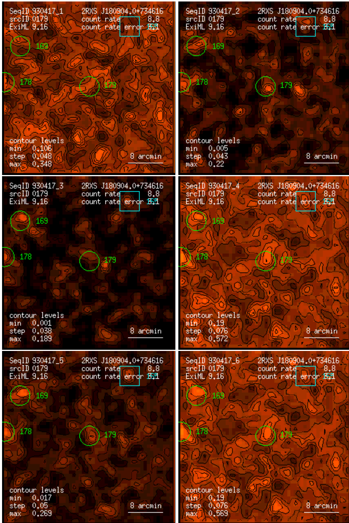
Figure 179: RASS 930417: detection 0179: band rate images, Gaussian filter: (1) PSPC channels 11 – 41, (2) 52 – 90, (3) 91 – 201, (4) 11 – 235, (5) 52 – 201, (6) 11 – 201. Broad band rates in counts/ks. Band rate contour levels in counts/ks/arcmin 2 .
