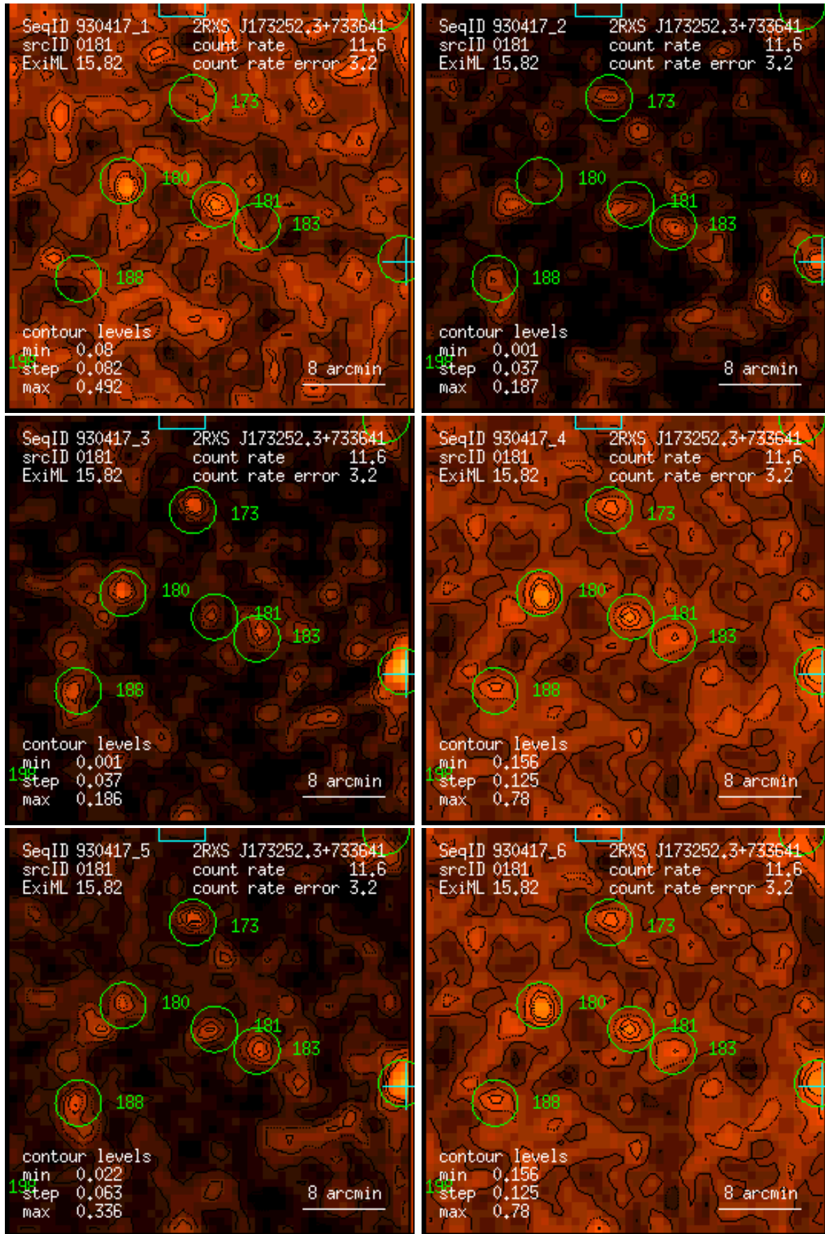
Figure 181: RASS 930417: detection 0181: band rate images, Gaussian filter: (1) PSPC channels 11 – 41, (2) 52 – 90, (3) 91 – 201, (4) 11 – 235, (5) 52 – 201, (6) 11 – 201. Broad band rates in counts/ks. Band rate contour levels in counts/ks/arcmin 2 .
