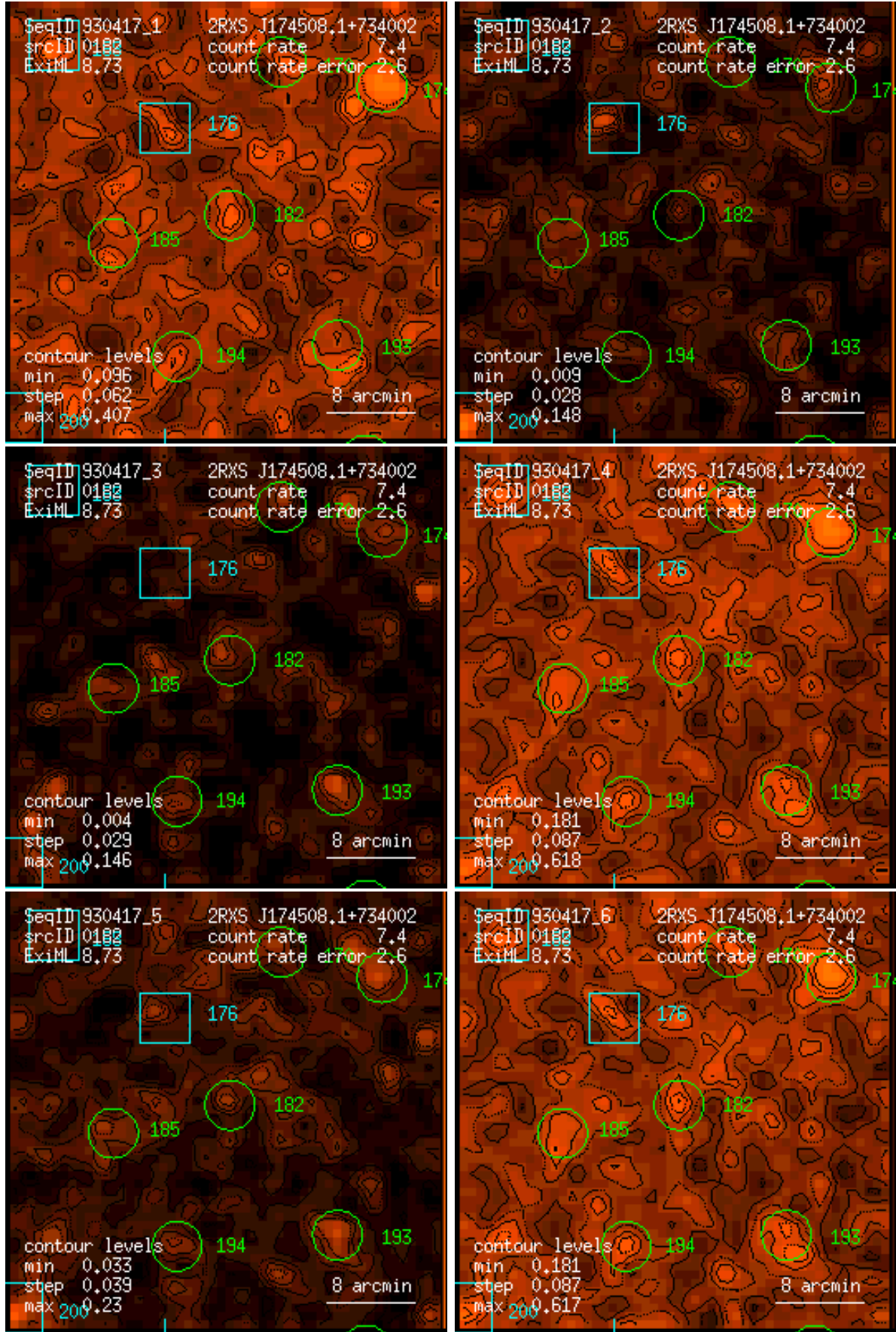
Figure 182: RASS 930417: detection 0182: band rate images, Gaussian filter: (1) PSPC channels 11 – 41, (2) 52 – 90, (3) 91 – 201, (4) 11 – 235, (5) 52 – 201, (6) 11 – 201. Broad band rates in counts/ks. Band rate contour levels in counts/ks/arcmin 2 .
