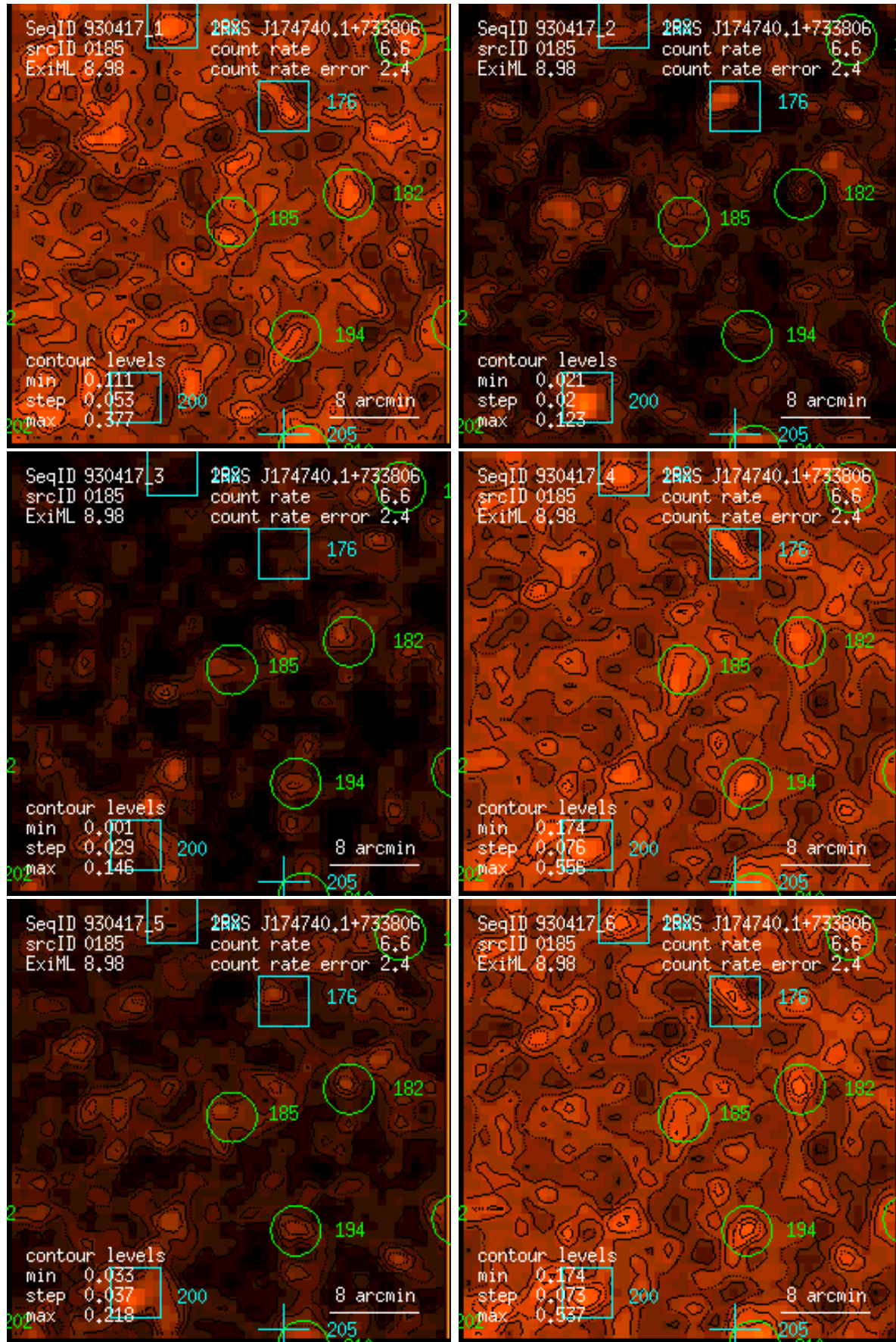
Figure 185: RASS 930417: detection 0185: band rate images, Gaussian filter: (1) PSPC channels 11 – 41, (2) 52 – 90, (3) 91 – 201, (4) 11 – 235, (5) 52 – 201, (6) 11 – 201. Broad band rates in counts/ks. Band rate contour levels in counts/ks/arcmin 2 .
