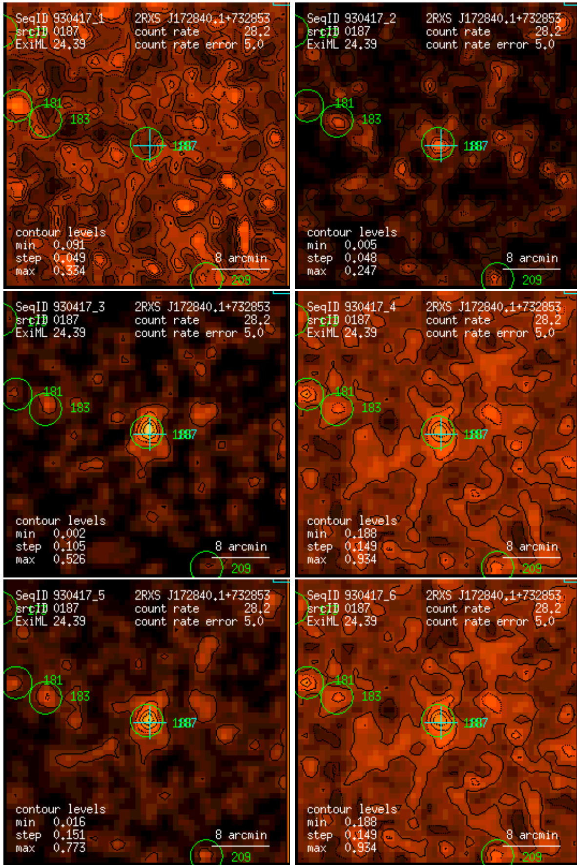
Figure 187: RASS 930417: detection 0187: band rate images, Gaussian filter: (1) PSPC channels 11 – 41, (2) 52 – 90, (3) 91 – 201, (4) 11 – 235, (5) 52 – 201, (6) 11 – 201. Broad band rates in counts/ks. Band rate contour levels in counts/ks/arcmin 2 .
