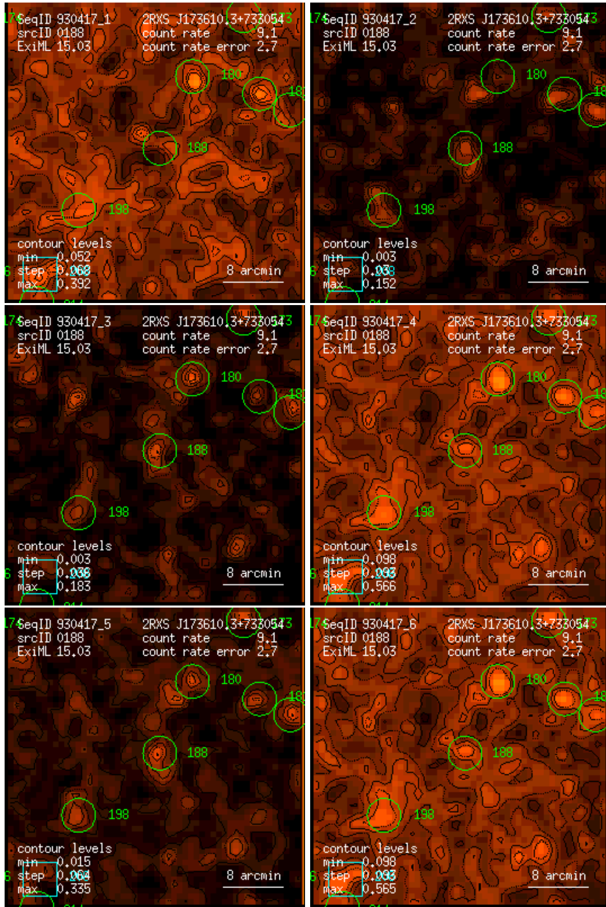
Figure 188: RASS 930417: detection 0188: band rate images, Gaussian filter: (1) PSPC channels 11 – 41, (2) 52 – 90, (3) 91 – 201, (4) 11 – 235, (5) 52 – 201, (6) 11 – 201. Broad band rates in counts/ks. Band rate contour levels in counts/ks/arcmin 2 .
