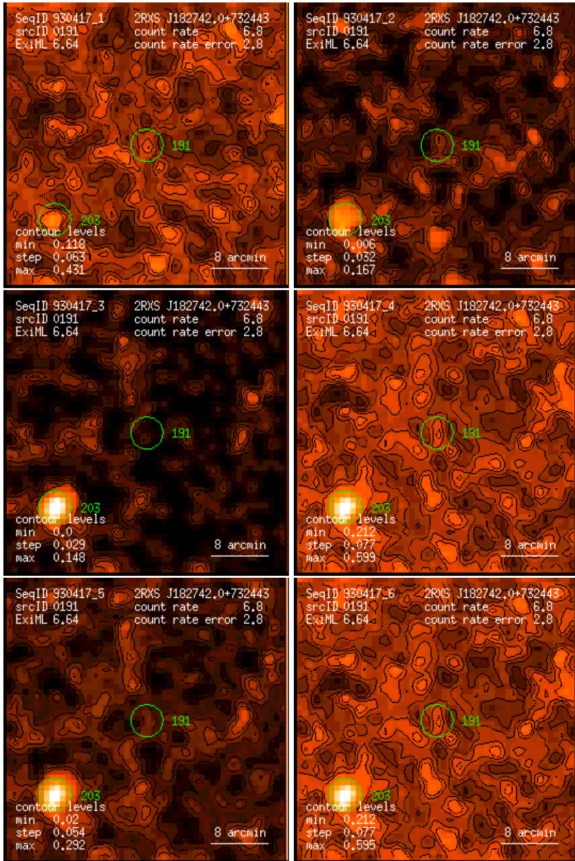
Figure 191: RASS 930417: detection 0191: band rate images, Gaussian filter: (1) PSPC channels 11 – 41, (2) 52 – 90, (3) 91 – 201, (4) 11 – 235, (5) 52 – 201, (6) 11 – 201. Broad band rates in counts/ks. Band rate contour levels in counts/ks/arcmin 2 .
