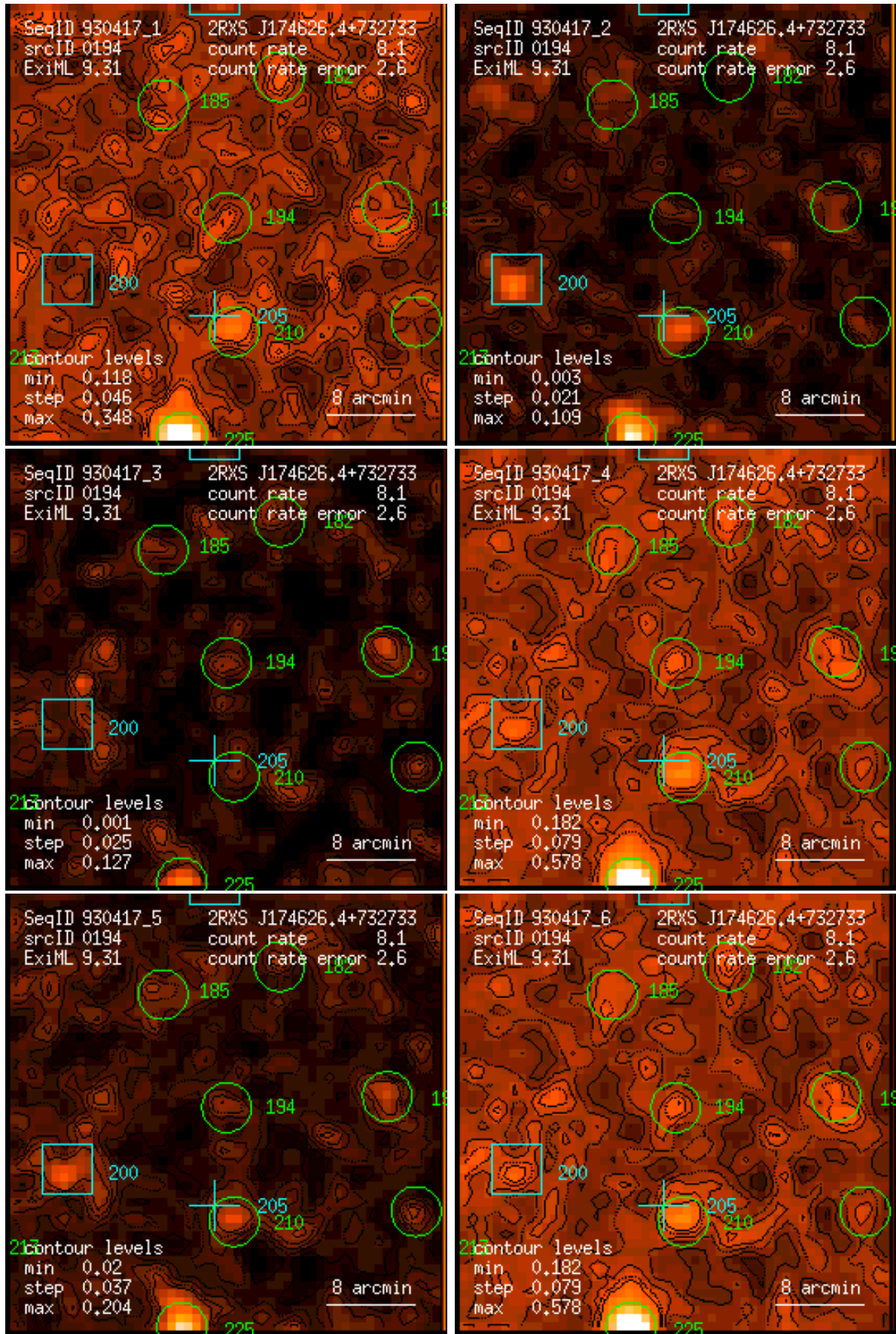
Figure 194: RASS 930417: detection 0194: band rate images, Gaussian filter: (1) PSPC channels 11 – 41, (2) 52 – 90, (3) 91 – 201, (4) 11 – 235, (5) 52 – 201, (6) 11 – 201. Broad band rates in counts/ks. Band rate contour levels in counts/ks/arcmin 2 .
