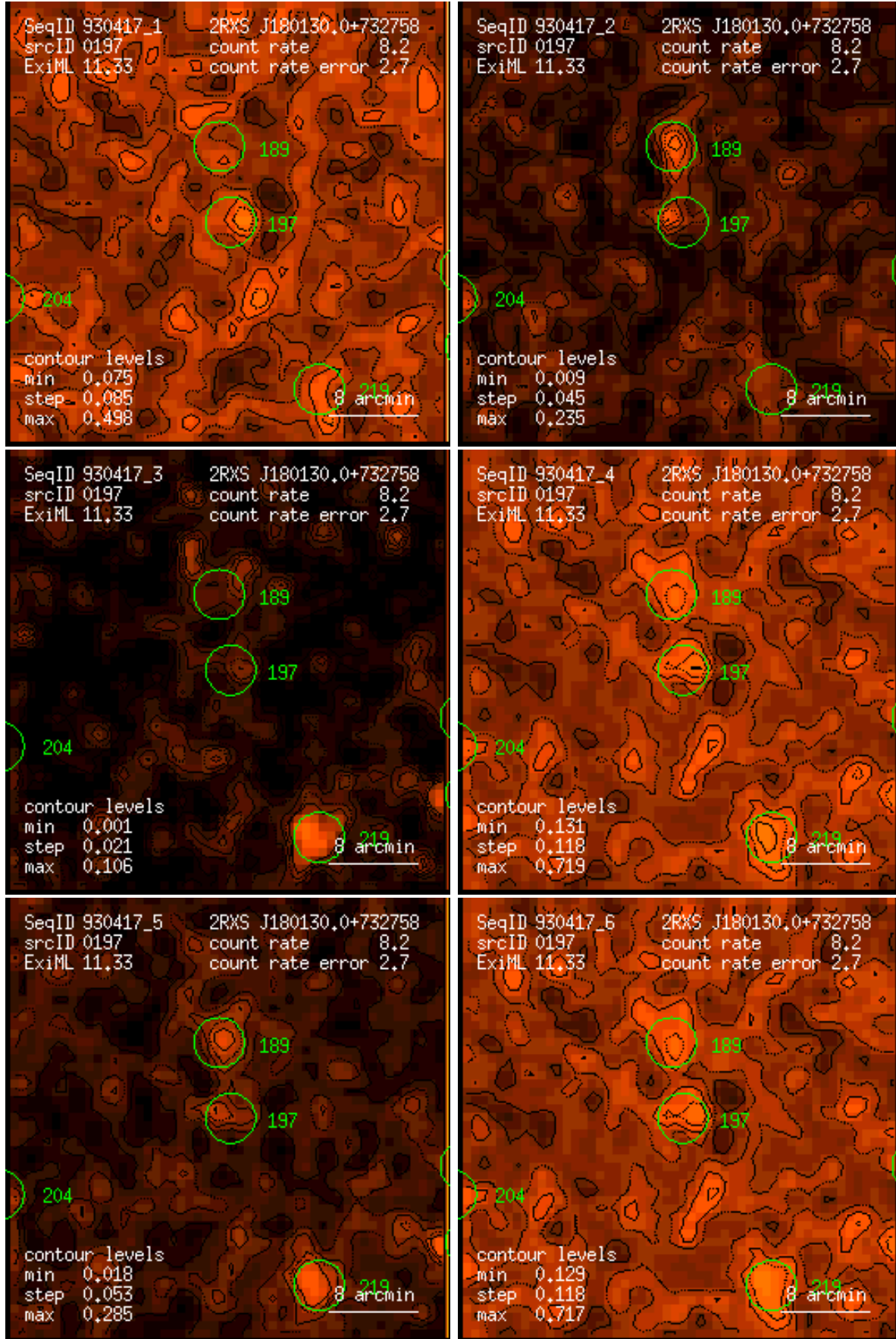
Figure 197: RASS 930417: detection 0197: band rate images, Gaussian filter: (1) PSPC channels 11 – 41, (2) 52 – 90, (3) 91 – 201, (4) 11 – 235, (5) 52 – 201, (6) 11 – 201. Broad band rates in counts/ks. Band rate contour levels in counts/ks/arcmin 2 .
