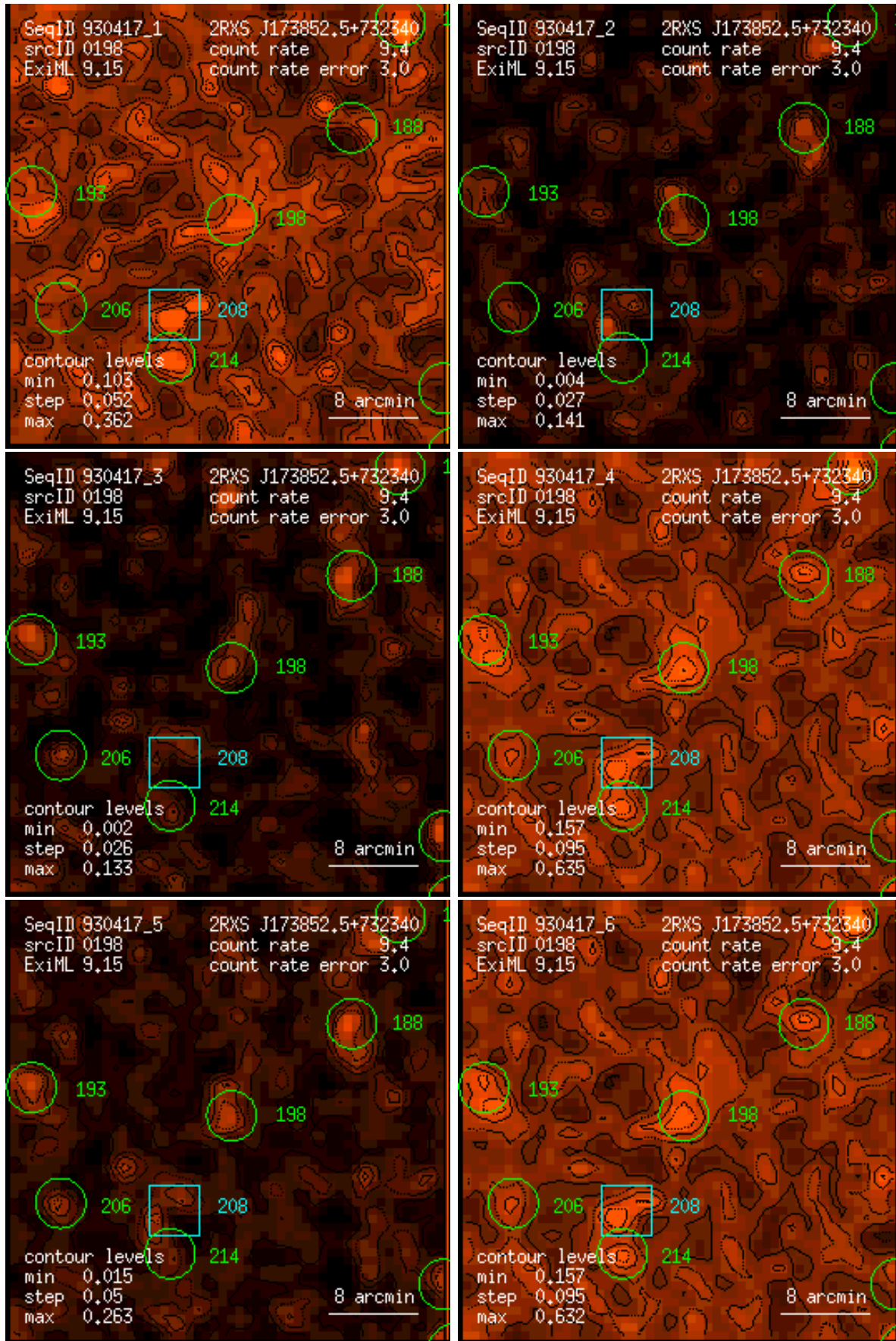
Figure 198: RASS 930417: detection 0198: band rate images, Gaussian filter: (1) PSPC channels 11 – 41, (2) 52 – 90, (3) 91 – 201, (4) 11 – 235, (5) 52 – 201, (6) 11 – 201. Broad band rates in counts/ks. Band rate contour levels in counts/ks/arcmin 2 .
