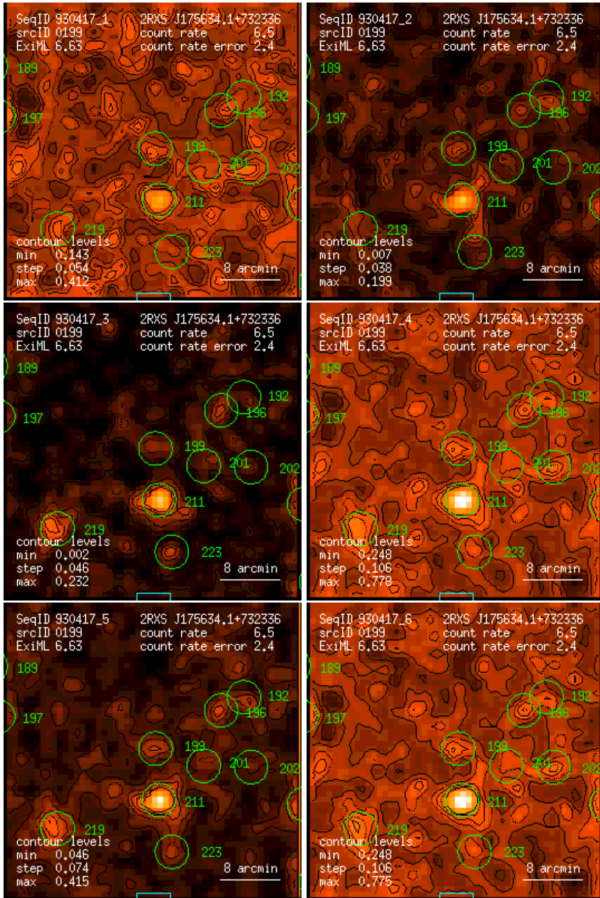
Figure 199: RASS 930417: detection 0199: band rate images, Gaussian filter: (1) PSPC channels 11 – 41, (2) 52 – 90, (3) 91 – 201, (4) 11 – 235, (5) 52 – 201, (6) 11 – 201. Broad band rates in counts/ks. Band rate contour levels in counts/ks/arcmin 2 .
