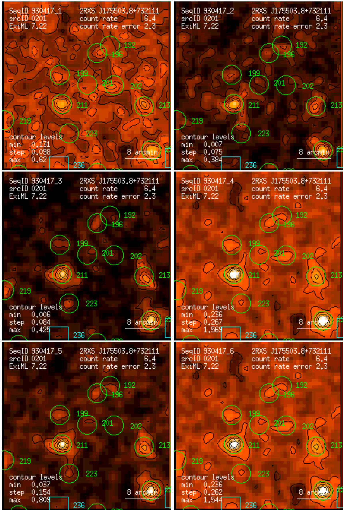
Figure 201: RASS 930417: detection 0201: band rate images, Gaussian filter: (1) PSPC channels 11 – 41, (2) 52 – 90, (3) 91 – 201, (4) 11 – 235, (5) 52 – 201, (6) 11 – 201. Broad band rates in counts/ks. Band rate contour levels in counts/ks/arcmin 2 .
