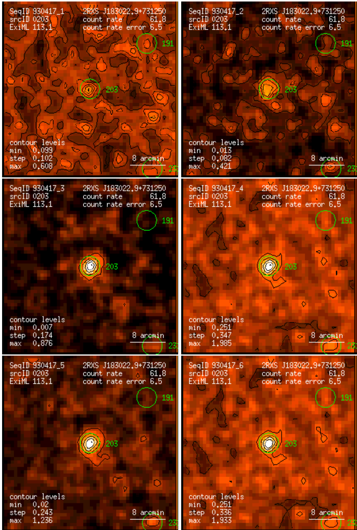
Figure 203: RASS 930417: detection 0203: band rate images, Gaussian filter: (1) PSPC channels 11 – 41, (2) 52 – 90, (3) 91 – 201, (4) 11 – 235, (5) 52 – 201, (6) 11 – 201. Broad band rates in counts/ks. Band rate contour levels in counts/ks/arcmin 2 .
