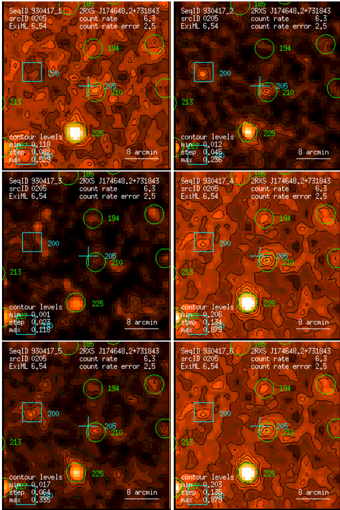
Figure 205: RASS 930417: detection 0205: band rate images, Gaussian filter: (1) PSPC channels 11 – 41, (2) 52 – 90, (3) 91 – 201, (4) 11 – 235, (5) 52 – 201, (6) 11 – 201. Broad band rates in counts/ks. Band rate contour levels in counts/ks/arcmin 2 .
