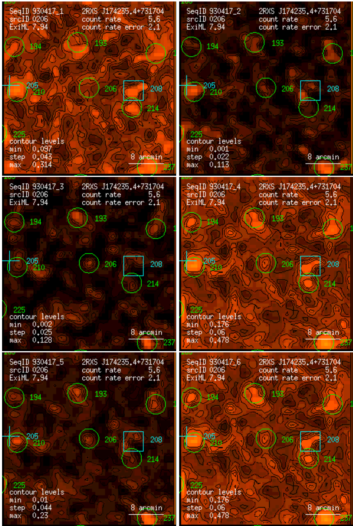
Figure 206: RASS 930417: detection 0206: band rate images, Gaussian filter: (1) PSPC channels 11 – 41, (2) 52 – 90, (3) 91 – 201, (4) 11 – 235, (5) 52 – 201, (6) 11 – 201. Broad band rates in counts/ks. Band rate contour levels in counts/ks/arcmin 2 .
