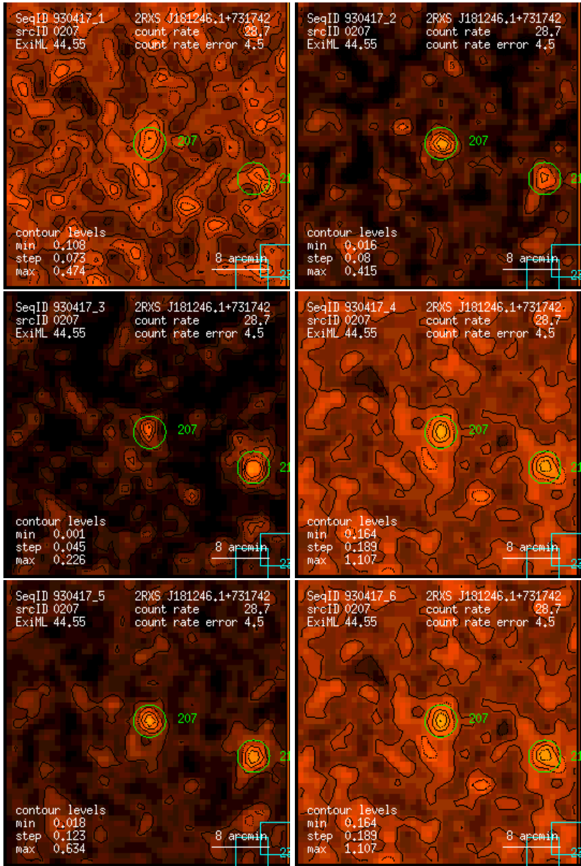
Figure 207: RASS 930417: detection 0207: band rate images, Gaussian filter: (1) PSPC channels 11 – 41, (2) 52 – 90, (3) 91 – 201, (4) 11 – 235, (5) 52 – 201, (6) 11 – 201. Broad band rates in counts/ks. Band rate contour levels in counts/ks/arcmin 2 .
