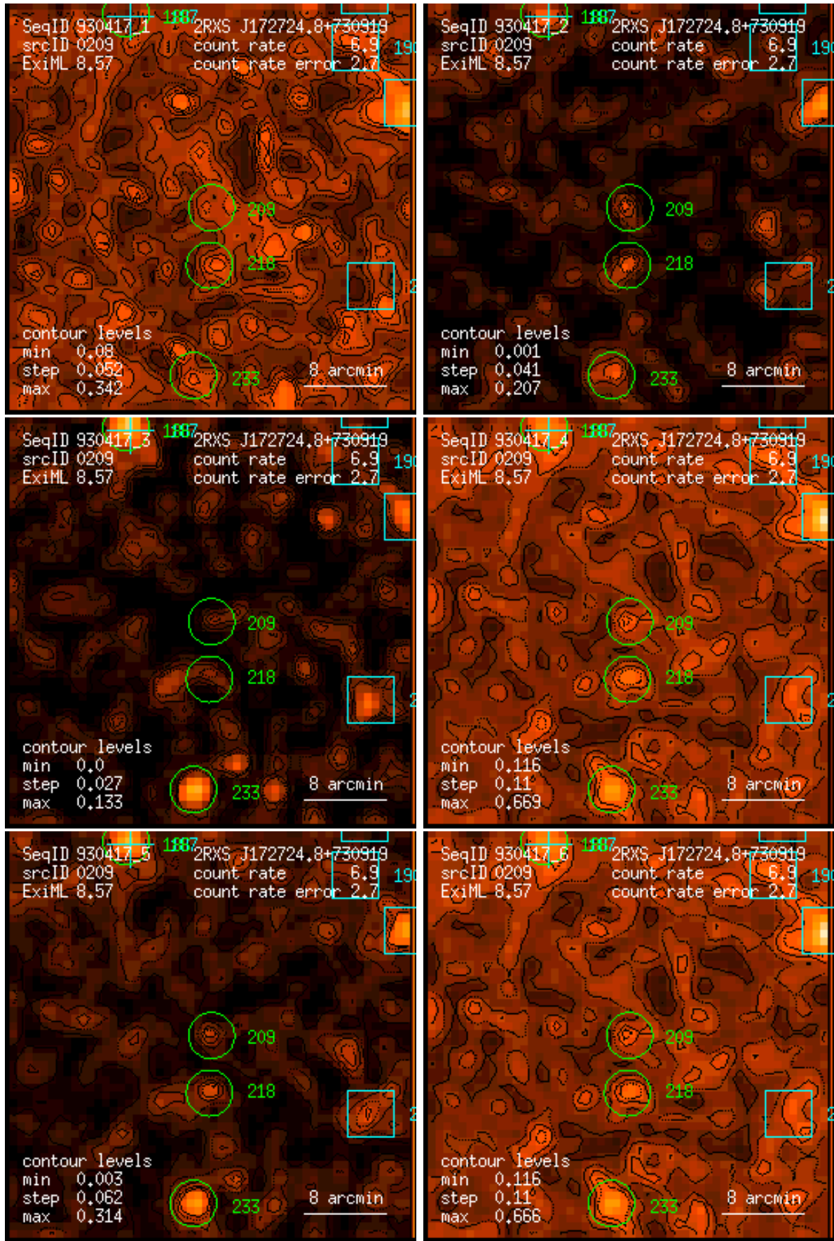
Figure 209: RASS 930417: detection 0209: band rate images, Gaussian filter: (1) PSPC channels 11 – 41, (2) 52 – 90, (3) 91 – 201, (4) 11 – 235, (5) 52 – 201, (6) 11 – 201. Broad band rates in counts/ks. Band rate contour levels in counts/ks/arcmin 2 .
