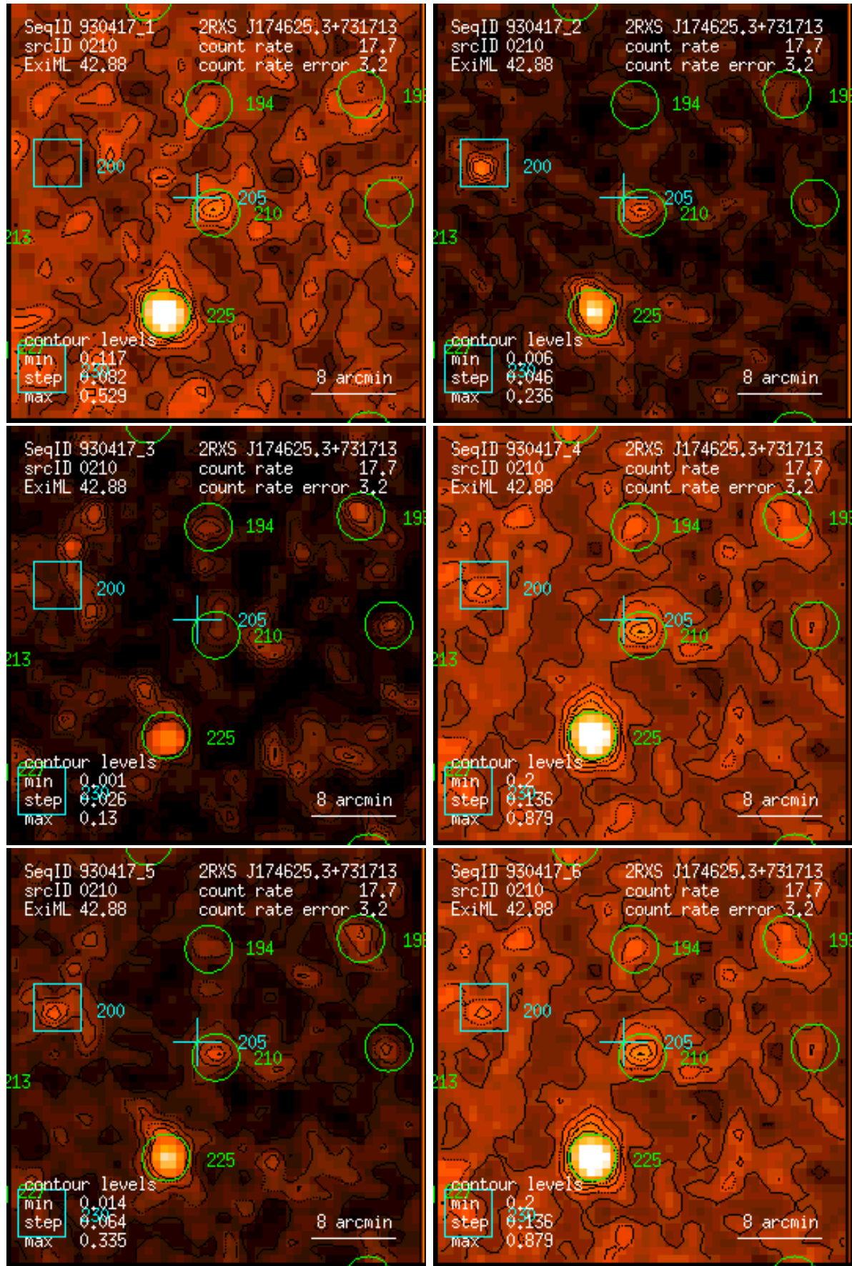
Figure 210: RASS 930417: detection 0210: band rate images, Gaussian filter: (1) PSPC channels 11 – 41, (2) 52 – 90, (3) 91 – 201, (4) 11 – 235, (5) 52 – 201, (6) 11 – 201. Broad band rates in counts/ks. Band rate contour levels in counts/ks/arcmin 2 .
