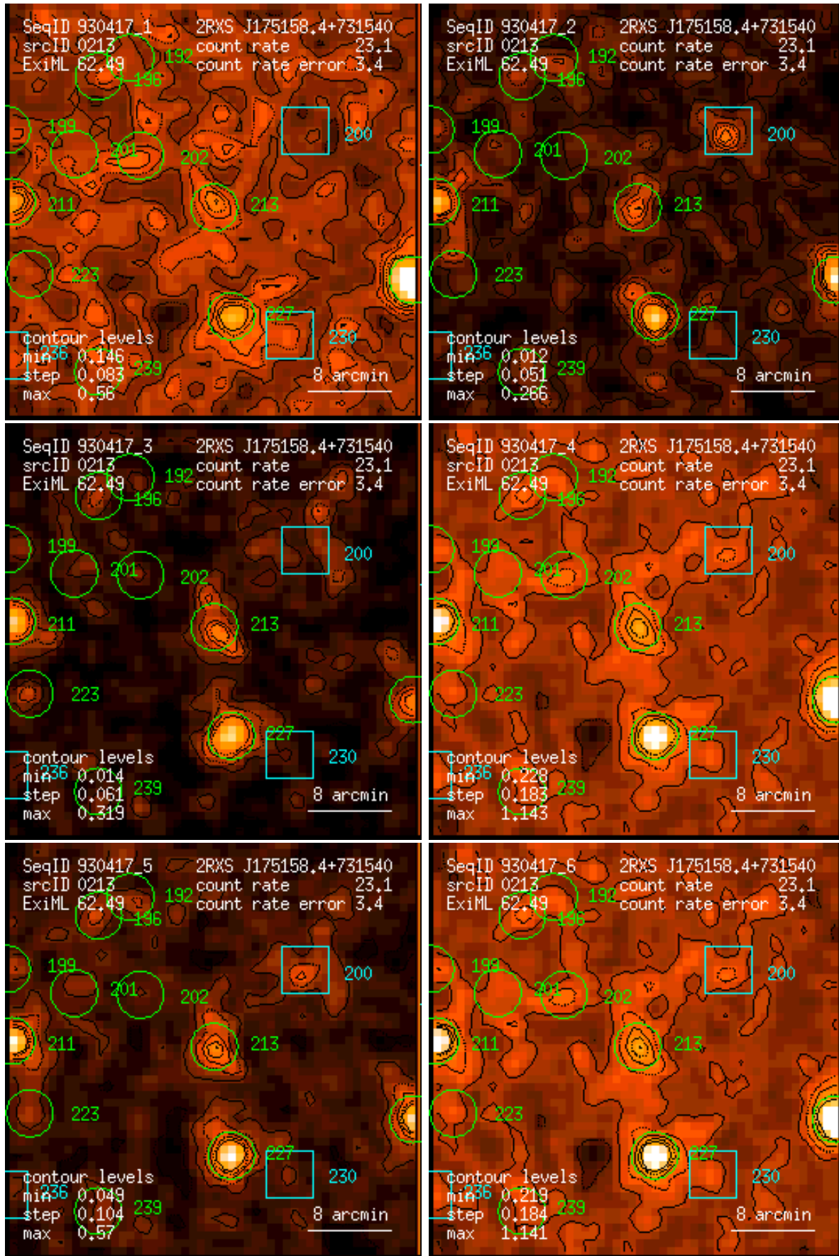
Figure 213: RASS 930417: detection 0213: band rate images, Gaussian filter: (1) PSPC channels 11 – 41, (2) 52 – 90, (3) 91 – 201, (4) 11 – 235, (5) 52 – 201, (6) 11 – 201. Broad band rates in counts/ks. Band rate contour levels in counts/ks/arcmin 2 .
