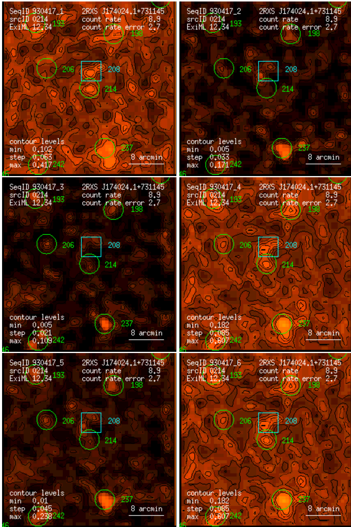
Figure 214: RASS 930417: detection 0214: band rate images, Gaussian filter: (1) PSPC channels 11 – 41, (2) 52 – 90, (3) 91 – 201, (4) 11 – 235, (5) 52 – 201, (6) 11 – 201. Broad band rates in counts/ks. Band rate contour levels in counts/ks/arcmin 2 .
