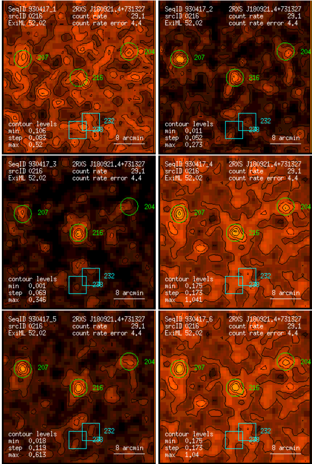
Figure 216: RASS 930417: detection 0216: band rate images, Gaussian filter: (1) PSPC channels 11 – 41, (2) 52 – 90, (3) 91 – 201, (4) 11 – 235, (5) 52 – 201, (6) 11 – 201. Broad band rates in counts/ks. Band rate contour levels in counts/ks/arcmin 2 .
