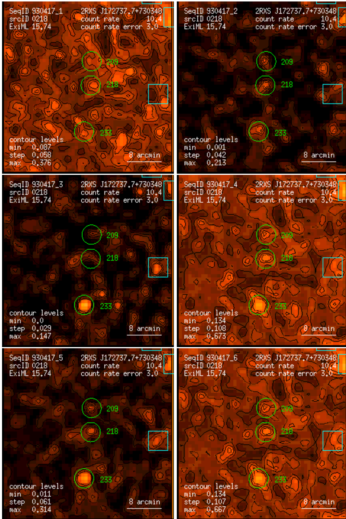
Figure 218: RASS 930417: detection 0218: band rate images, Gaussian filter: (1) PSPC channels 11 – 41, (2) 52 – 90, (3) 91 – 201, (4) 11 – 235, (5) 52 – 201, (6) 11 – 201. Broad band rates in counts/ks. Band rate contour levels in counts/ks/arcmin 2 .
