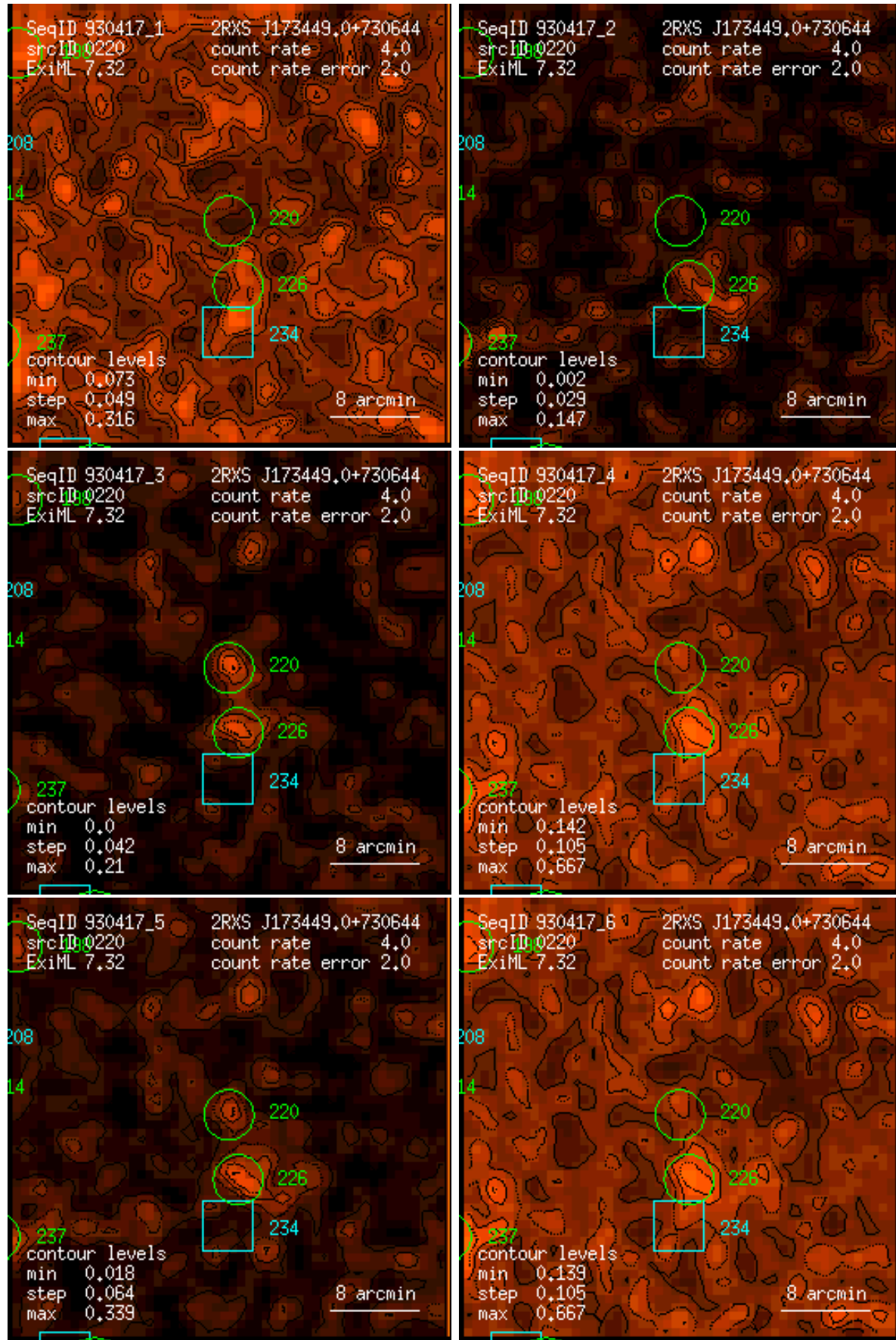
Figure 220: RASS 930417: detection 0220: band rate images, Gaussian filter: (1) PSPC channels 11 – 41, (2) 52 – 90, (3) 91 – 201, (4) 11 – 235, (5) 52 – 201, (6) 11 – 201. Broad band rates in counts/ks. Band rate contour levels in counts/ks/arcmin 2 .
