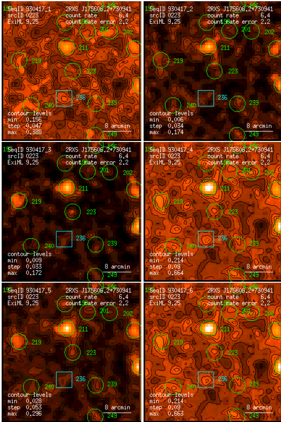
Figure 223: RASS 930417: detection 0223: band rate images, Gaussian filter: (1) PSPC channels 11 – 41, (2) 52 – 90, (3) 91 – 201, (4) 11 – 235, (5) 52 – 201, (6) 11 – 201. Broad band rates in counts/ks. Band rate contour levels in counts/ks/arcmin 2 .
