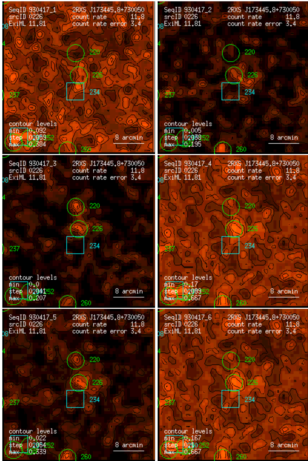
Figure 226: RASS 930417: detection 0226: band rate images, Gaussian filter: (1) PSPC channels 11 – 41, (2) 52 – 90, (3) 91 – 201, (4) 11 – 235, (5) 52 – 201, (6) 11 – 201. Broad band rates in counts/ks. Band rate contour levels in counts/ks/arcmin 2 .
