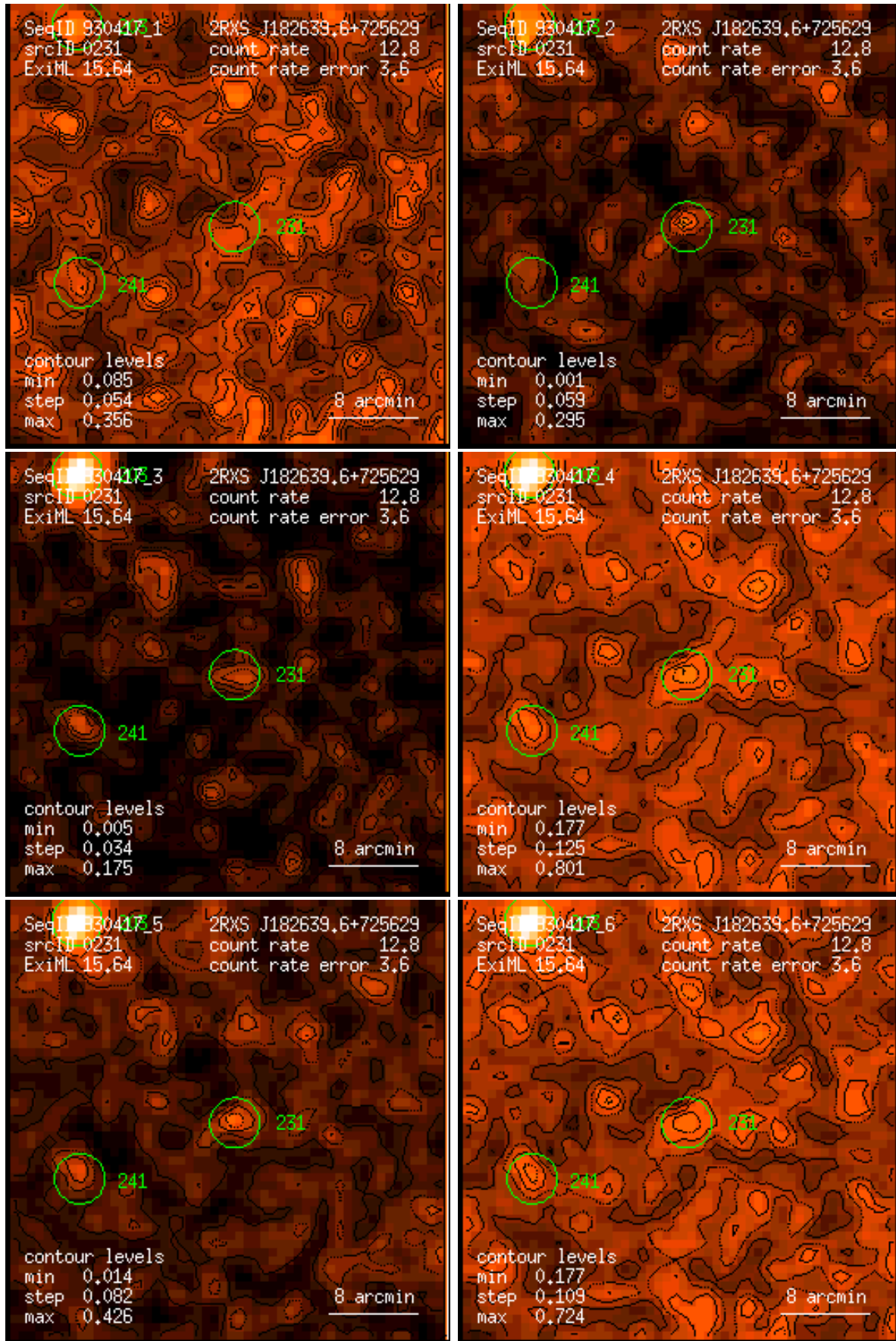
Figure 231: RASS 930417: detection 0231: band rate images, Gaussian filter: (1) PSPC channels 11 – 41, (2) 52 – 90, (3) 91 – 201, (4) 11 – 235, (5) 52 – 201, (6) 11 – 201. Broad band rates in counts/ks. Band rate contour levels in counts/ks/arcmin 2 .
