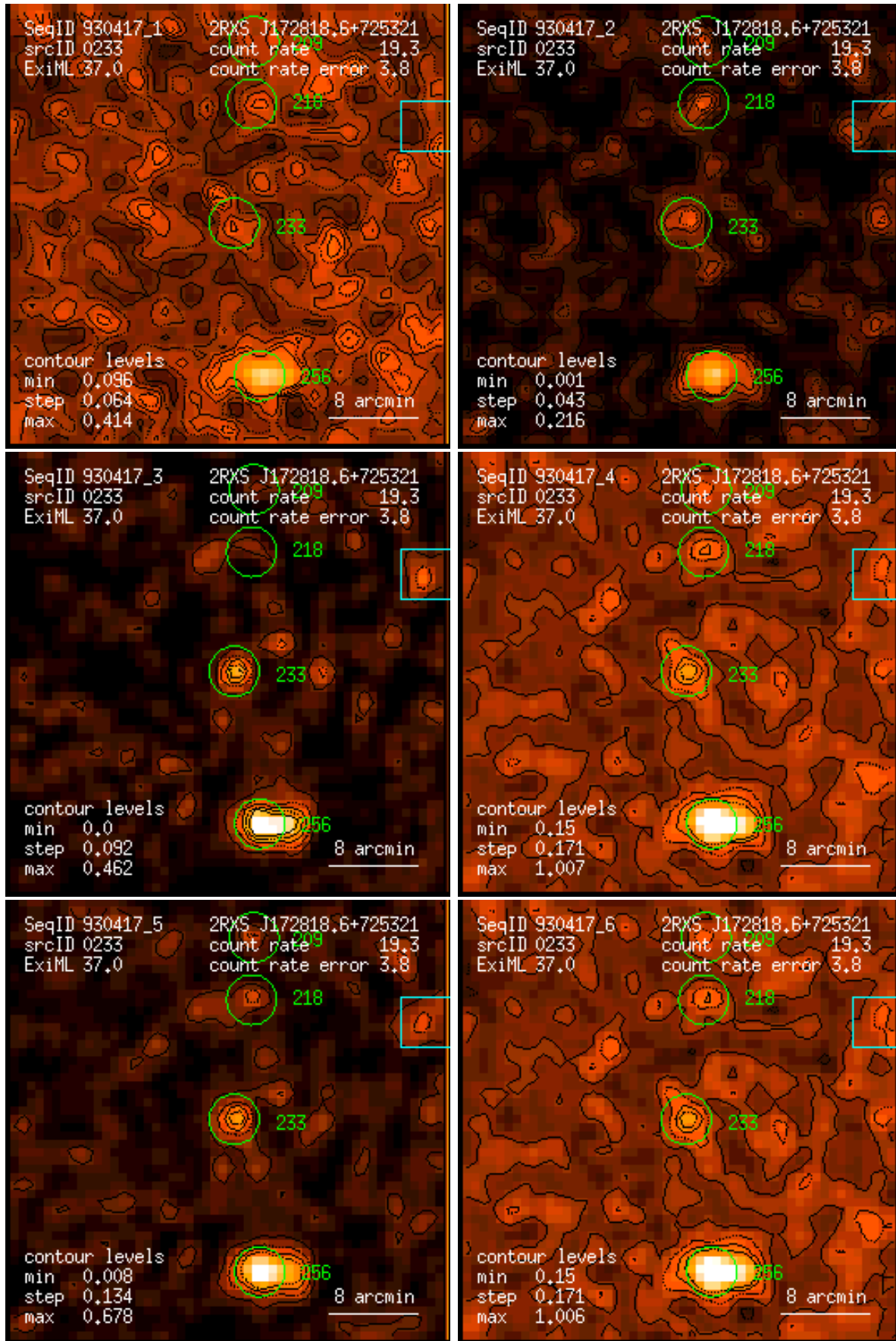
Figure 233: RASS 930417: detection 0233: band rate images, Gaussian filter: (1) PSPC channels 11 – 41, (2) 52 – 90, (3) 91 – 201, (4) 11 – 235, (5) 52 – 201, (6) 11 – 201. Broad band rates in counts/ks. Band rate contour levels in counts/ks/arcmin 2 .
