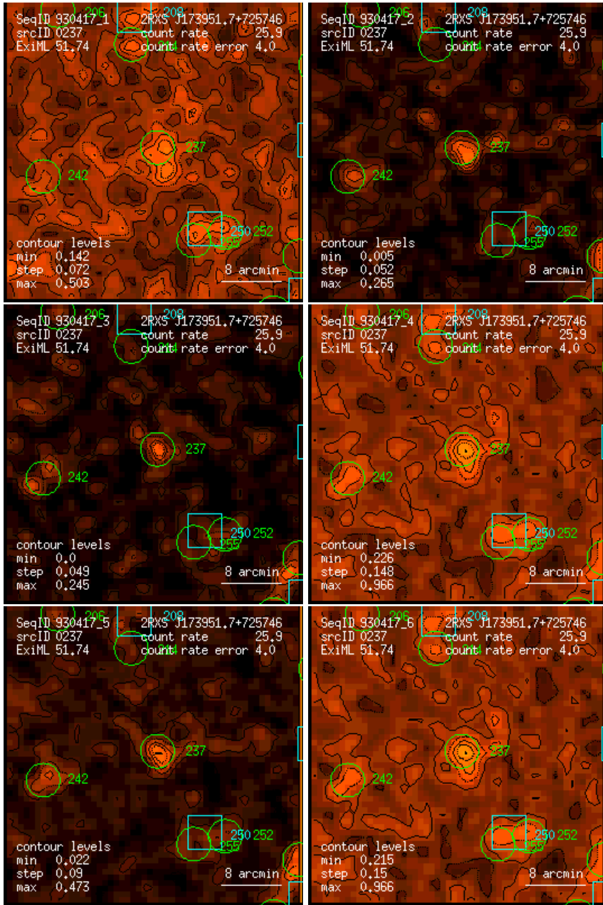
Figure 237: RASS 930417: detection 0237: band rate images, Gaussian filter: (1) PSPC channels 11 – 41, (2) 52 – 90, (3) 91 – 201, (4) 11 – 235, (5) 52 – 201, (6) 11 – 201. Broad band rates in counts/ks. Band rate contour levels in counts/ks/arcmin 2 .
