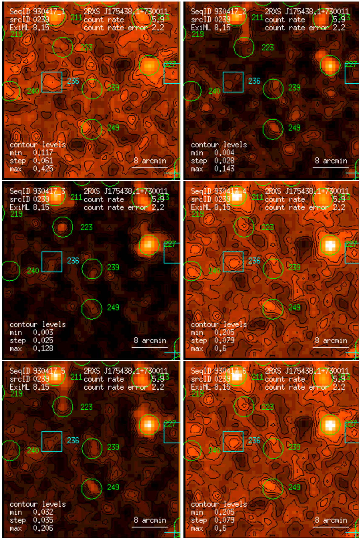
Figure 239: RASS 930417: detection 0239: band rate images, Gaussian filter: (1) PSPC channels 11 – 41, (2) 52 – 90, (3) 91 – 201, (4) 11 – 235, (5) 52 – 201, (6) 11 – 201. Broad band rates in counts/ks. Band rate contour levels in counts/ks/arcmin 2 .
