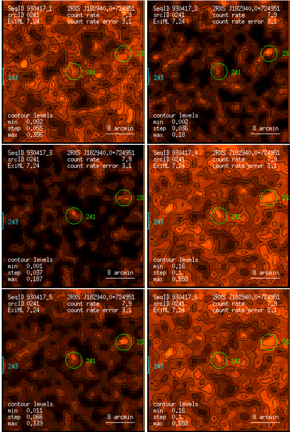
Figure 241: RASS 930417: detection 0241: band rate images, Gaussian filter: (1) PSPC channels 11 – 41, (2) 52 – 90, (3) 91 – 201, (4) 11 – 235, (5) 52 – 201, (6) 11 – 201. Broad band rates in counts/ks. Band rate contour levels in counts/ks/arcmin 2 .
