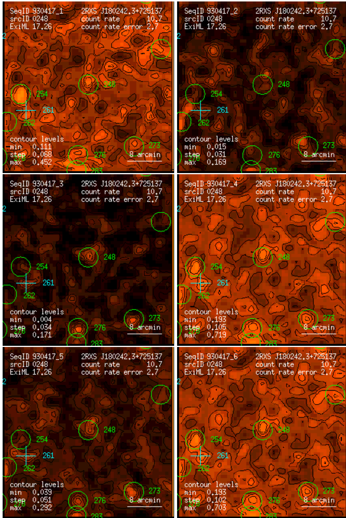
Figure 248: RASS 930417: detection 0248: band rate images, Gaussian filter: (1) PSPC channels 11 – 41, (2) 52 – 90, (3) 91 – 201, (4) 11 – 235, (5) 52 – 201, (6) 11 – 201. Broad band rates in counts/ks. Band rate contour levels in counts/ks/arcmin 2 .
