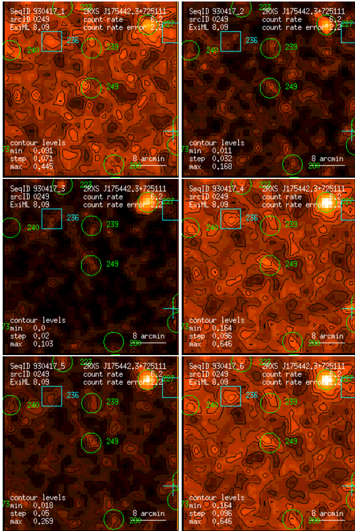
Figure 249: RASS 930417: detection 0249: band rate images, Gaussian filter: (1) PSPC channels 11 – 41, (2) 52 – 90, (3) 91 – 201, (4) 11 – 235, (5) 52 – 201, (6) 11 – 201. Broad band rates in counts/ks. Band rate contour levels in counts/ks/arcmin 2 .
