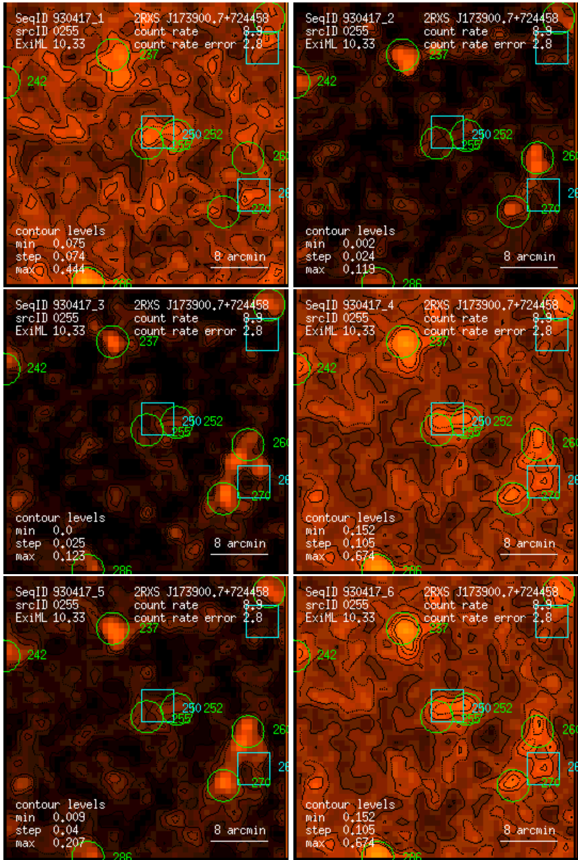
Figure 255: RASS 930417: detection 0255: band rate images, Gaussian filter: (1) PSPC channels 11 – 41, (2) 52 – 90, (3) 91 – 201, (4) 11 – 235, (5) 52 – 201, (6) 11 – 201. Broad band rates in counts/ks. Band rate contour levels in counts/ks/arcmin 2 .
