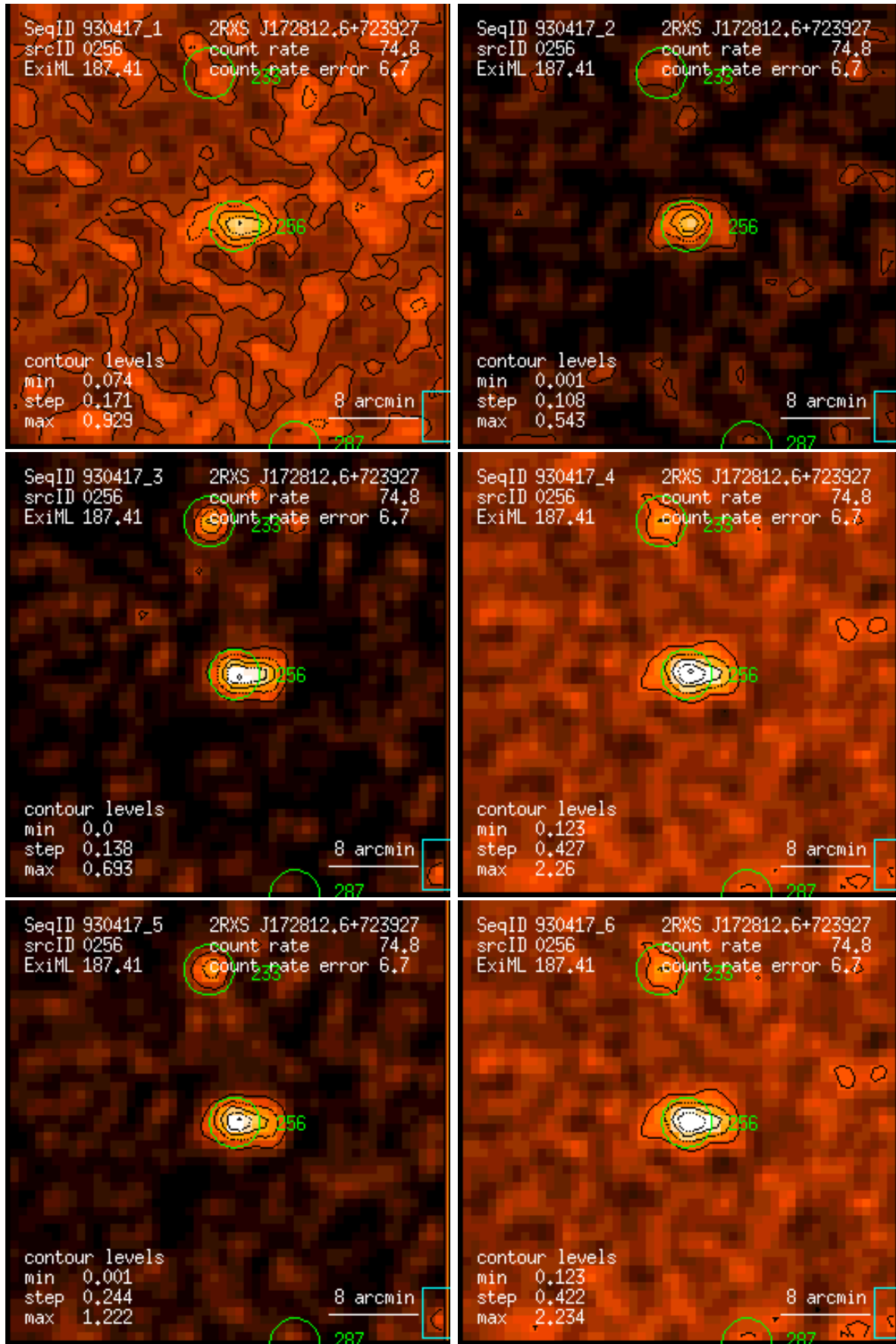
Figure 256: RASS 930417: detection 0256: band rate images, Gaussian filter: (1) PSPC channels 11 – 41, (2) 52 – 90, (3) 91 – 201, (4) 11 – 235, (5) 52 – 201, (6) 11 – 201. Broad band rates in counts/ks. Band rate contour levels in counts/ks/arcmin 2 .
