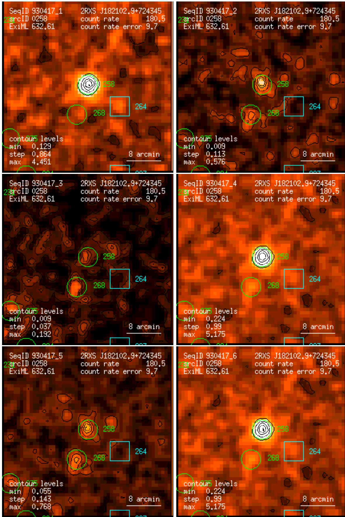
Figure 258: RASS 930417: detection 0258: band rate images, Gaussian filter: (1) PSPPC channels 11 – 41, (2) 52 – 90, (3) 91 – 201, (4) 11 – 235, (5) 52 – 201, (6) 11 – 201. Broad band rates in counts/ks. Band rate contour levels in counts/ks/arcmin 2 .
