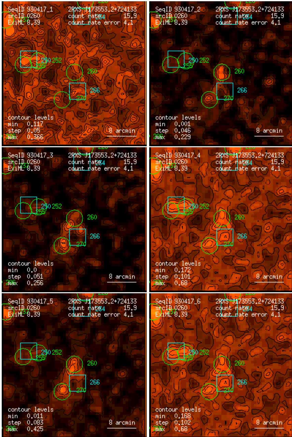
Figure 260: RASS 930417: detection 0260: band rate images, Gaussian filter: (1) PSPC channels 11 – 41, (2) 52 – 90, (3) 91 – 201, (4) 11 – 235, (5) 52 – 201, (6) 11 – 201. Broad band rates in counts/ks. Band rate contour levels in counts/ks/arcmin 2 .
