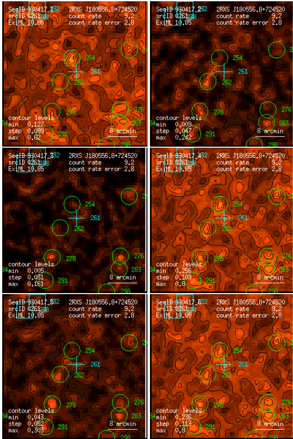
Figure 261: RASS 930417: detection 0261: band rate images, Gaussian filter: (1) PSPC channels 11 – 41, (2) 52 – 90, (3) 91 – 201, (4) 11 – 235, (5) 52 – 201, (6) 11 – 201. Broad band rates in counts/ks. Band rate contour levels in counts/ks/arcmin 2 .
