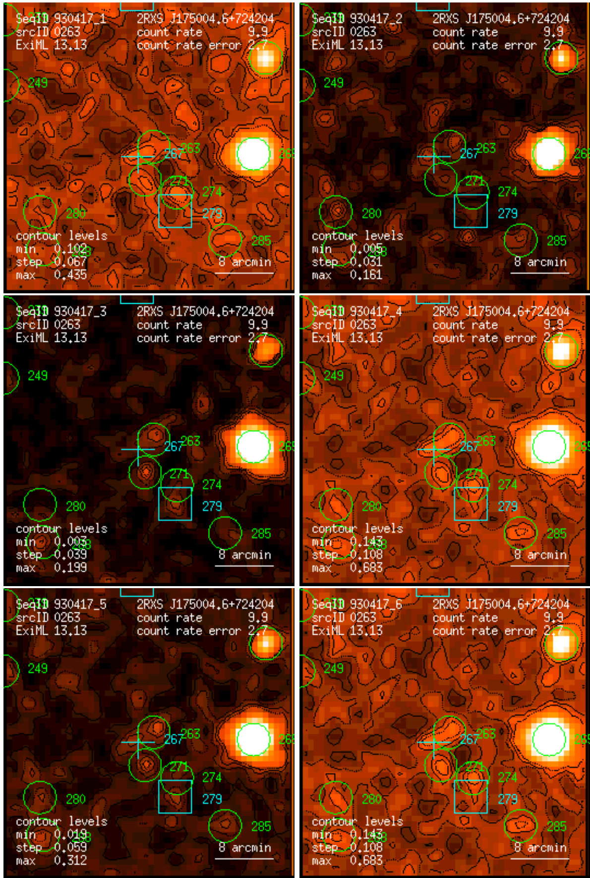
Figure 263: RASS 930417: detection 0263: band rate images, Gaussian filter: (1) PSPC channels 11 – 41, (2) 52 – 90, (3) 91 – 201, (4) 11 – 235, (5) 52 – 201, (6) 11 – 201. Broad band rates in counts/ks. Band rate contour levels in counts/ks/arcmin 2 .
