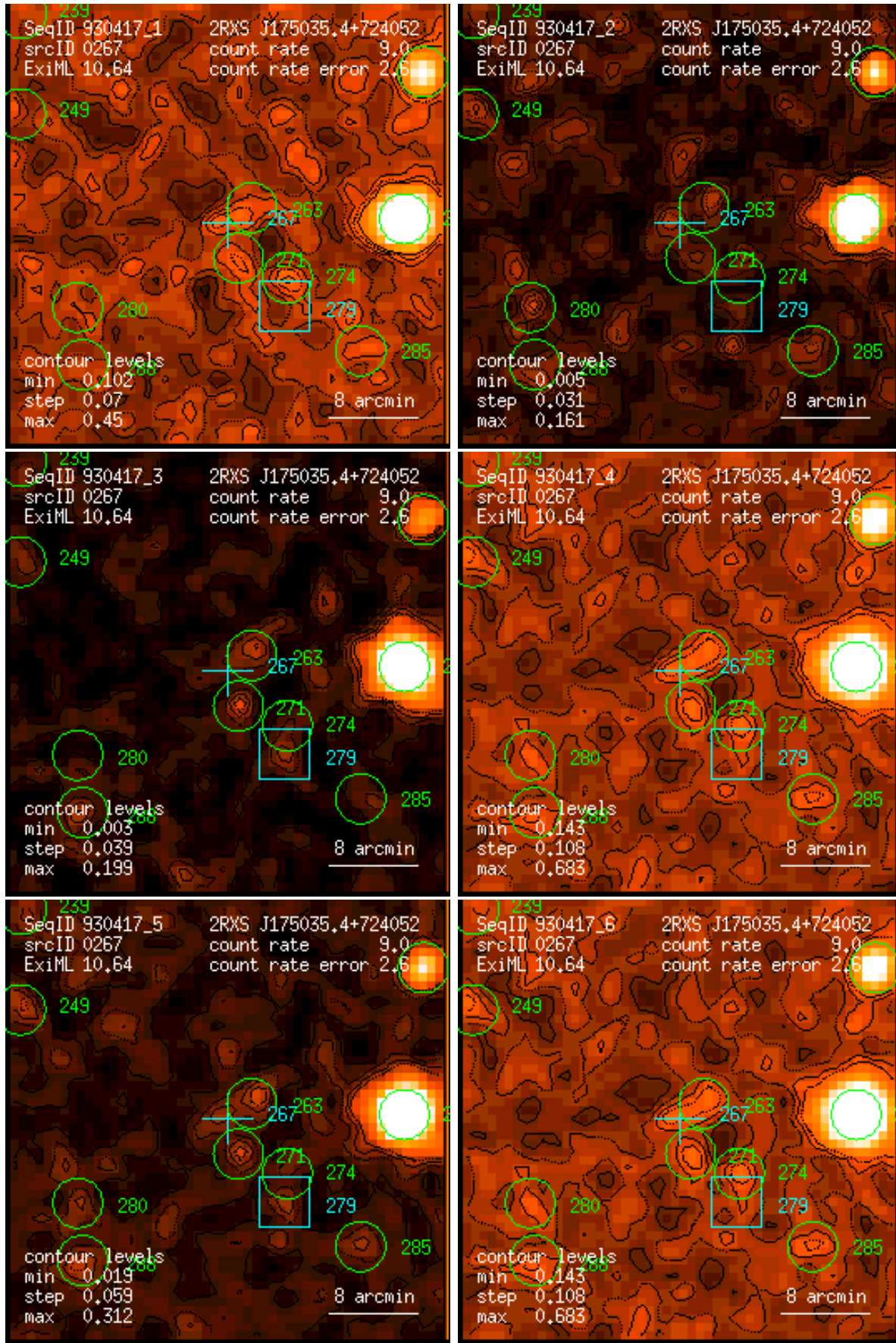
Figure 267: RASS 930417: detection 0267: band rate images, Gaussian filter: (1) PSPC channels 11 – 41, (2) 52 – 90, (3) 91 – 201, (4) 11 – 235, (5) 52 – 201, (6) 11 – 201. Broad band rates in counts/ks. Band rate contour levels in counts/ks/arcmin 2 .
