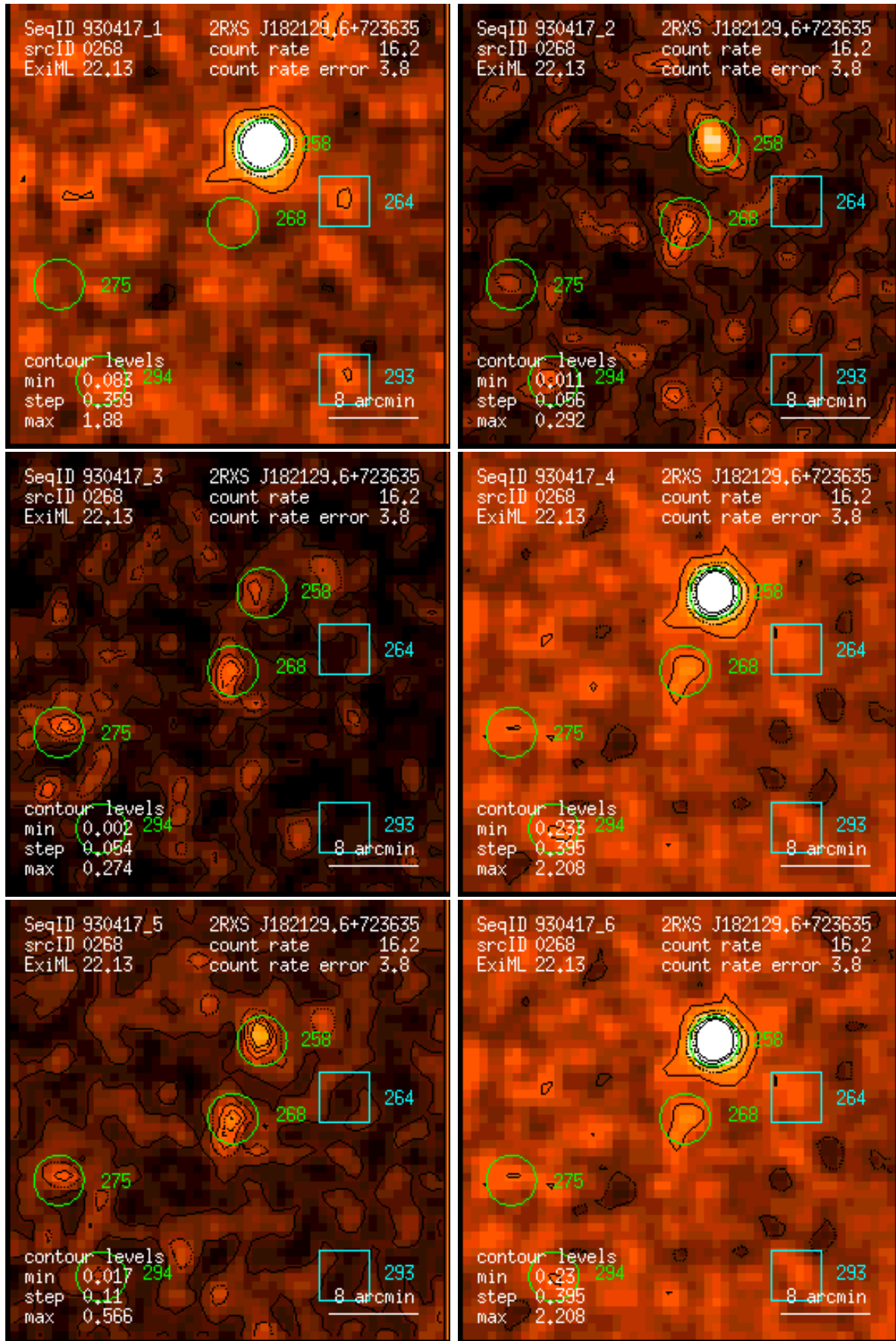
Figure 268: RASS 930417: detection 0268: band rate images, Gaussian filter: (1) PSPC channels 11 – 41, (2) 52 – 90, (3) 91 – 201, (4) 11 – 235, (5) 52 – 201, (6) 11 – 201. Broad band rates in counts/ks. Band rate contour levels in counts/ks/arcmin 2 .
